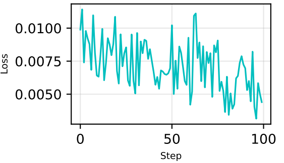
Student BC (outer iter 4)
