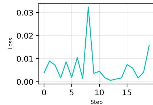
Student BC (outer iter 7)
