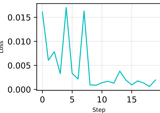
Student BC (outer iter 5)
