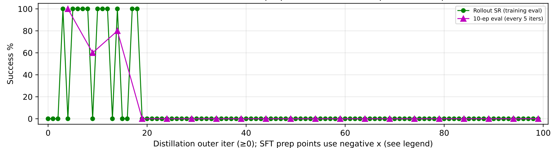
Student success rate: SFT prep eval, rollout distill, periodic 10-ep
