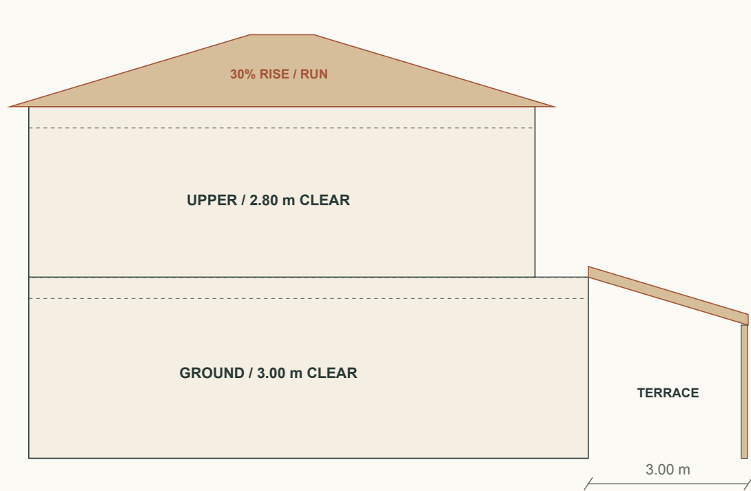
SIDE PROFILE / ROOF HEIGHT ADDED SEPARATELY
