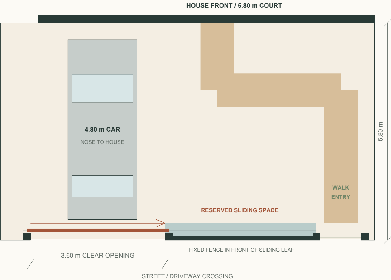
Gate dimensions / planning allowances
