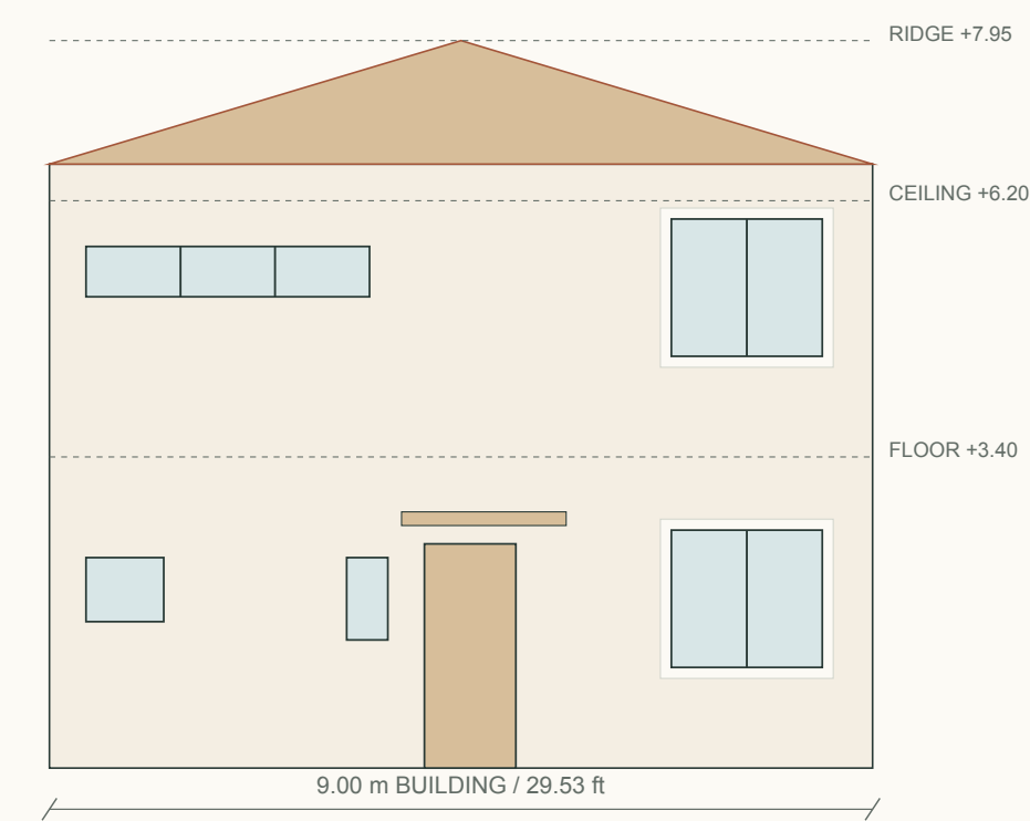
FRONT ELEVATION / OPENINGS IN THEIR ROOMS
