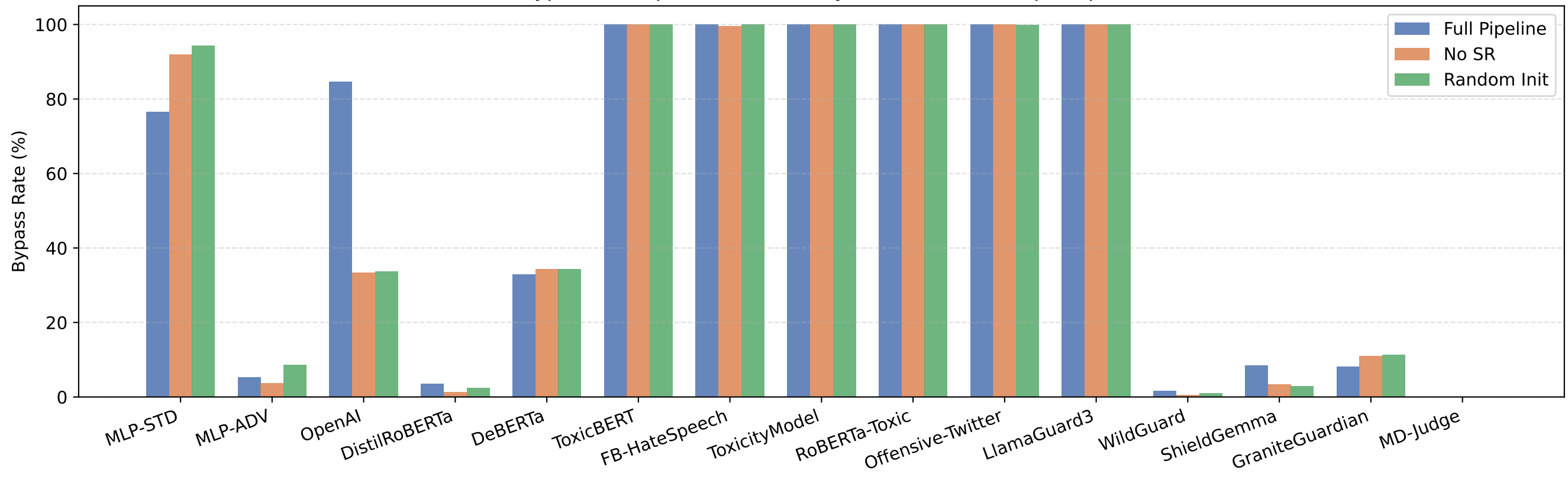
Bypass Rate per Moderation System - 1990 total prompts
