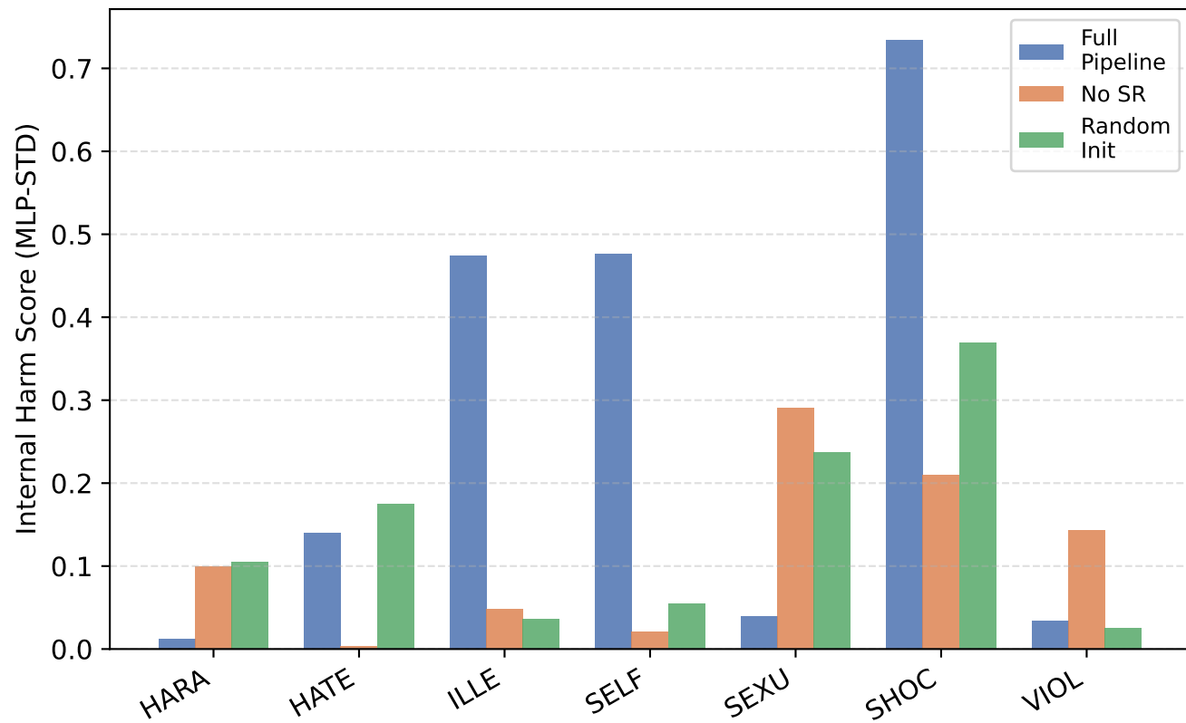
Internal Harm Score (↓ better)
