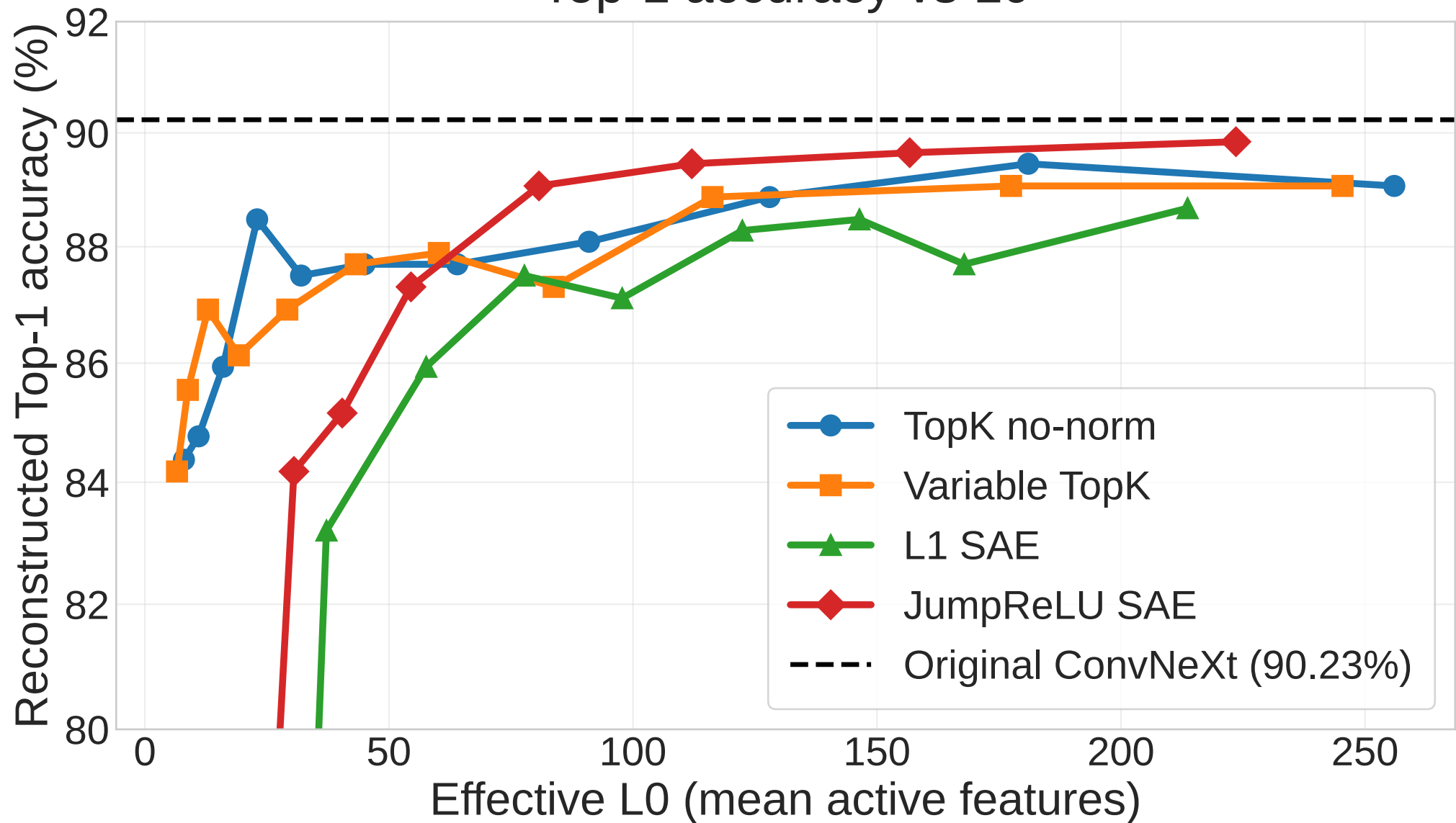
Top-1 accuracy vs L0
