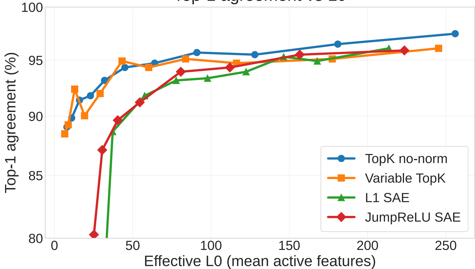
Top-1 agreement vs L0
