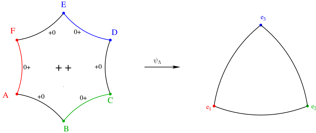
Figure 2.2: The extension of the Moser map, \psi_\Lambda .
