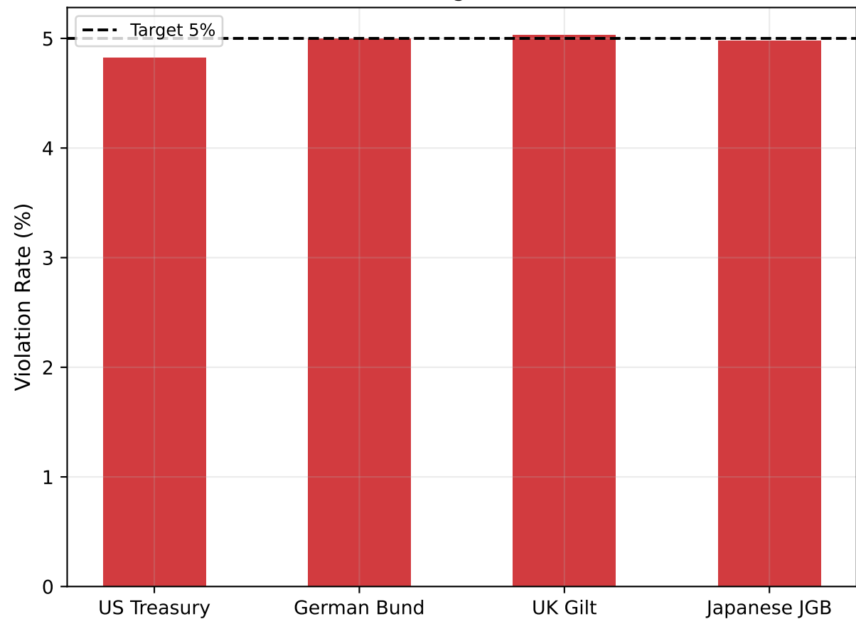
VaR Coverage (5% level)
