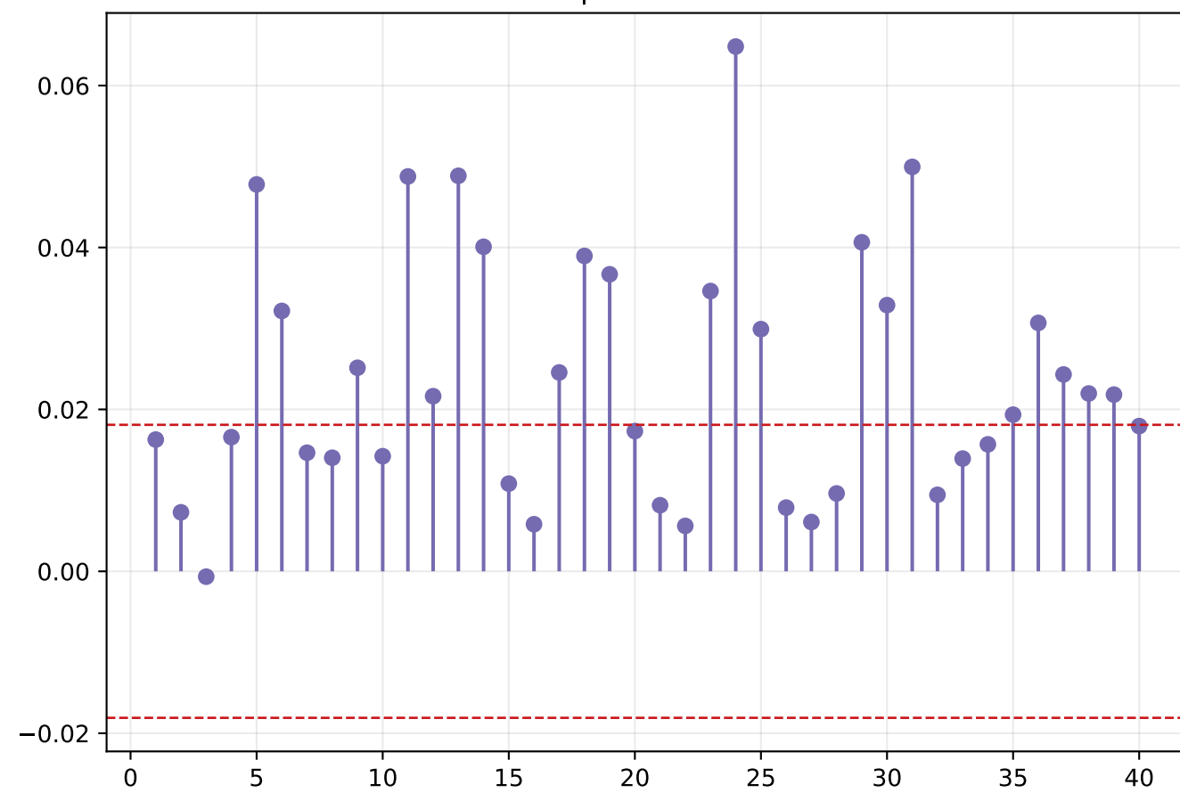
ACF: Squared Residuals
