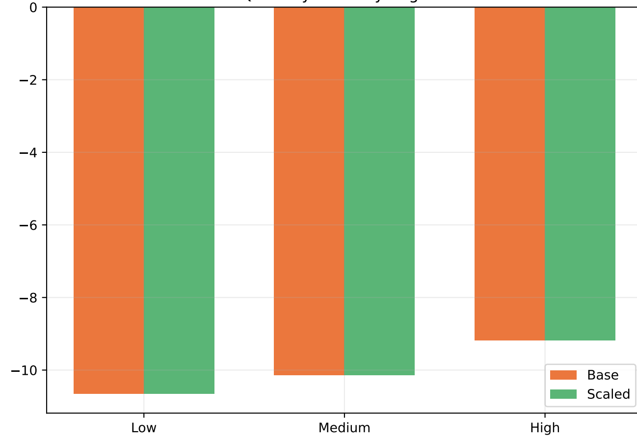
QLIKE by Volatility Regime
