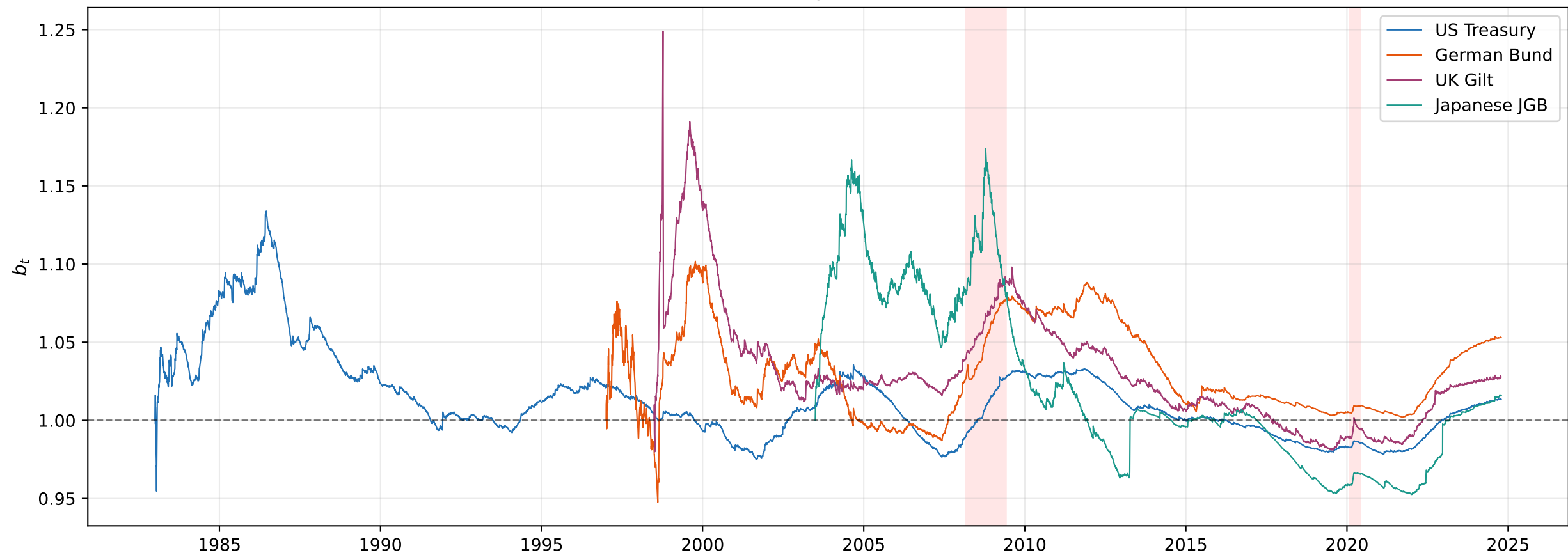
Variance-Level Multiplier b_t Across Markets
