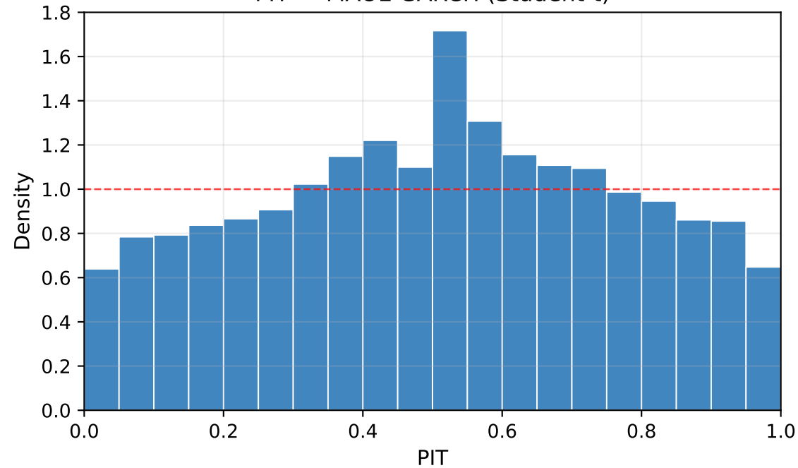
PIT — MAOL-GARCH (Student-t)
