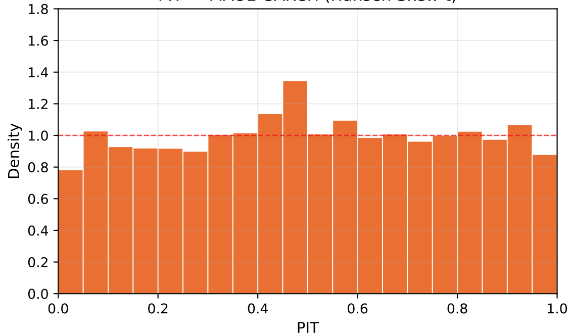
PIT — MAOL-GARCH (Hansen Skew-t)
