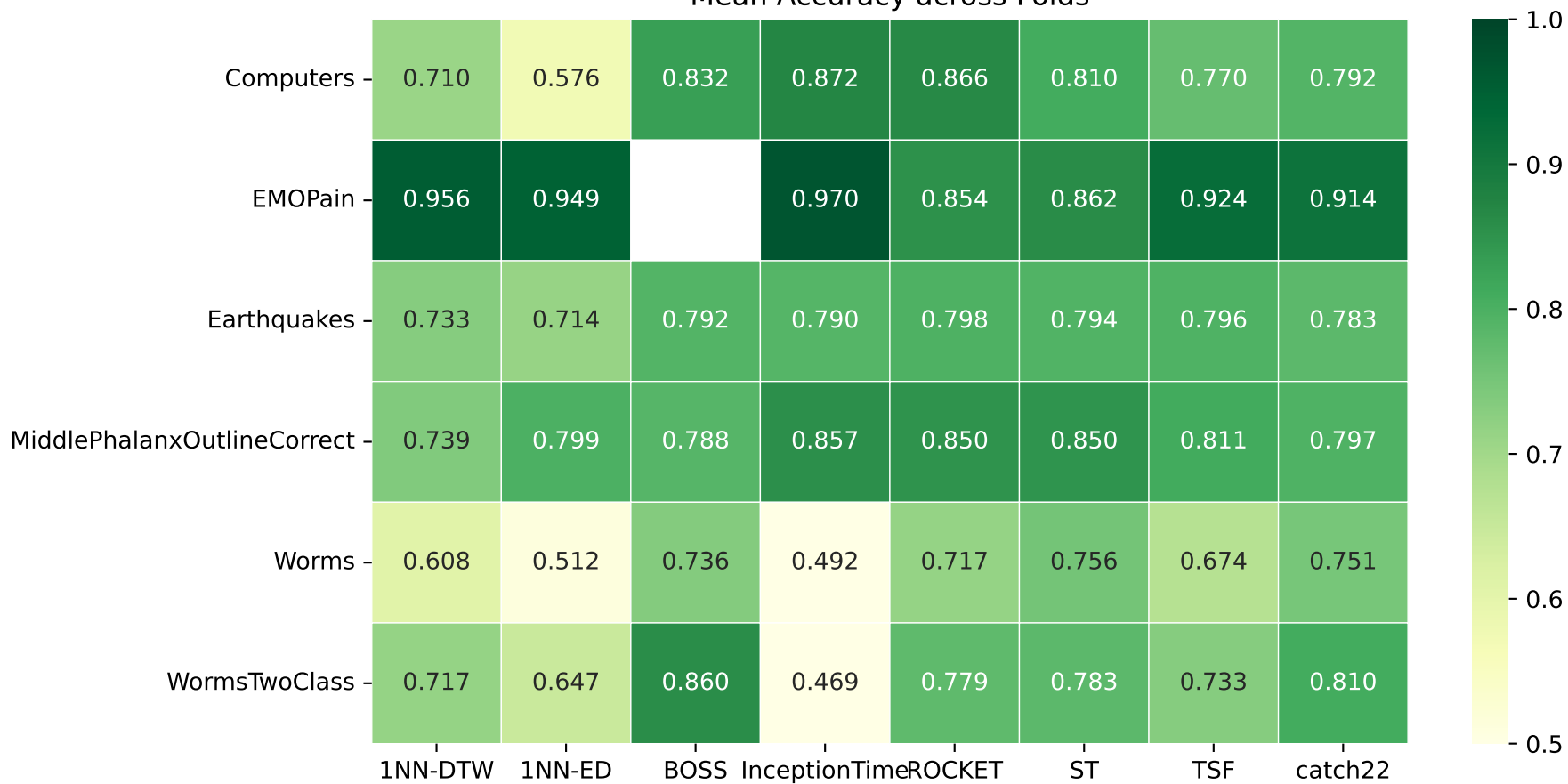
Mean Accuracy across Folds
