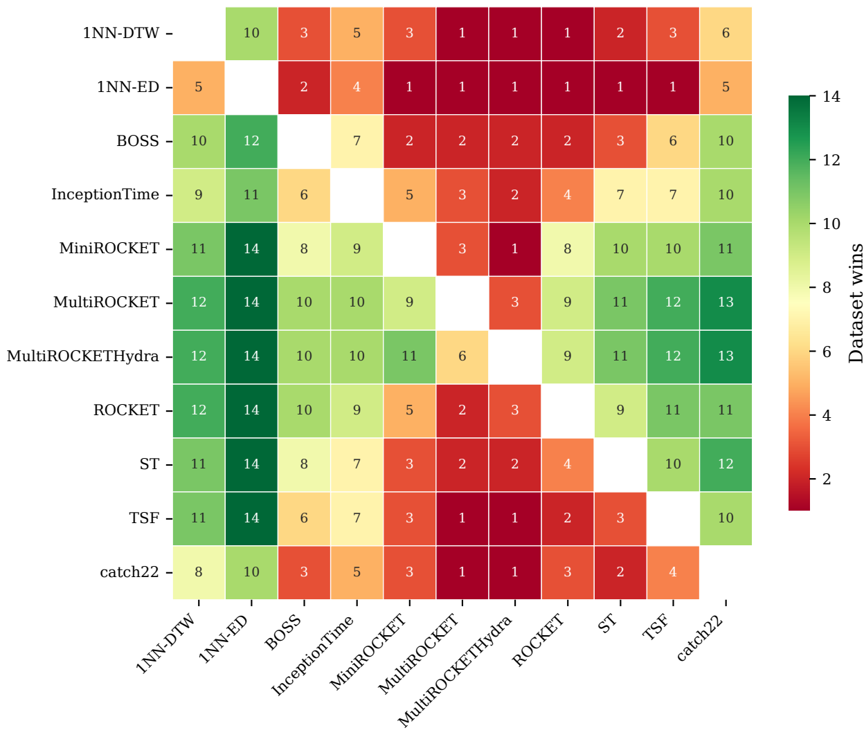
Pairwise Dataset Wins (row beats column)
