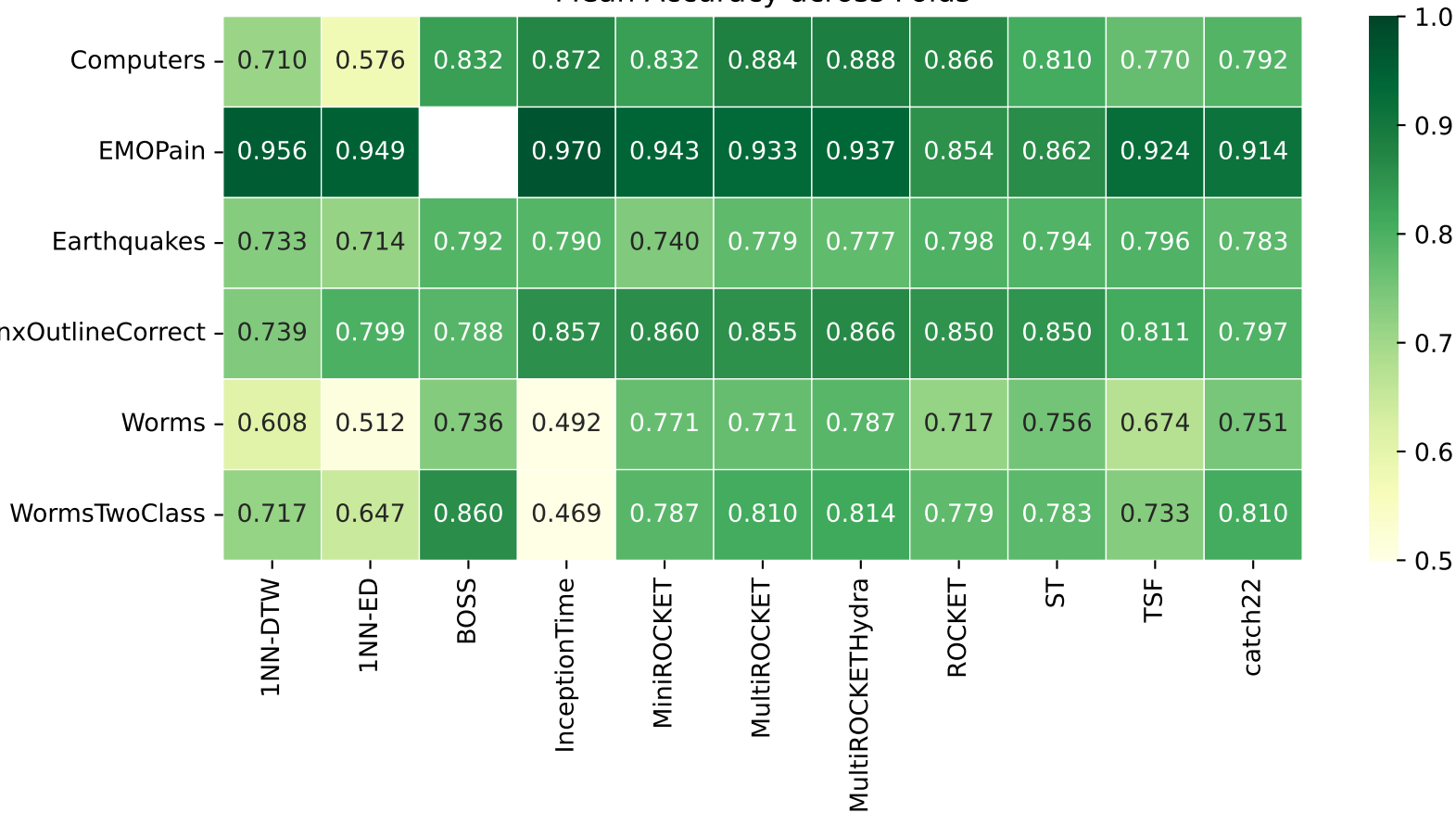
Mean Accuracy across Folds
