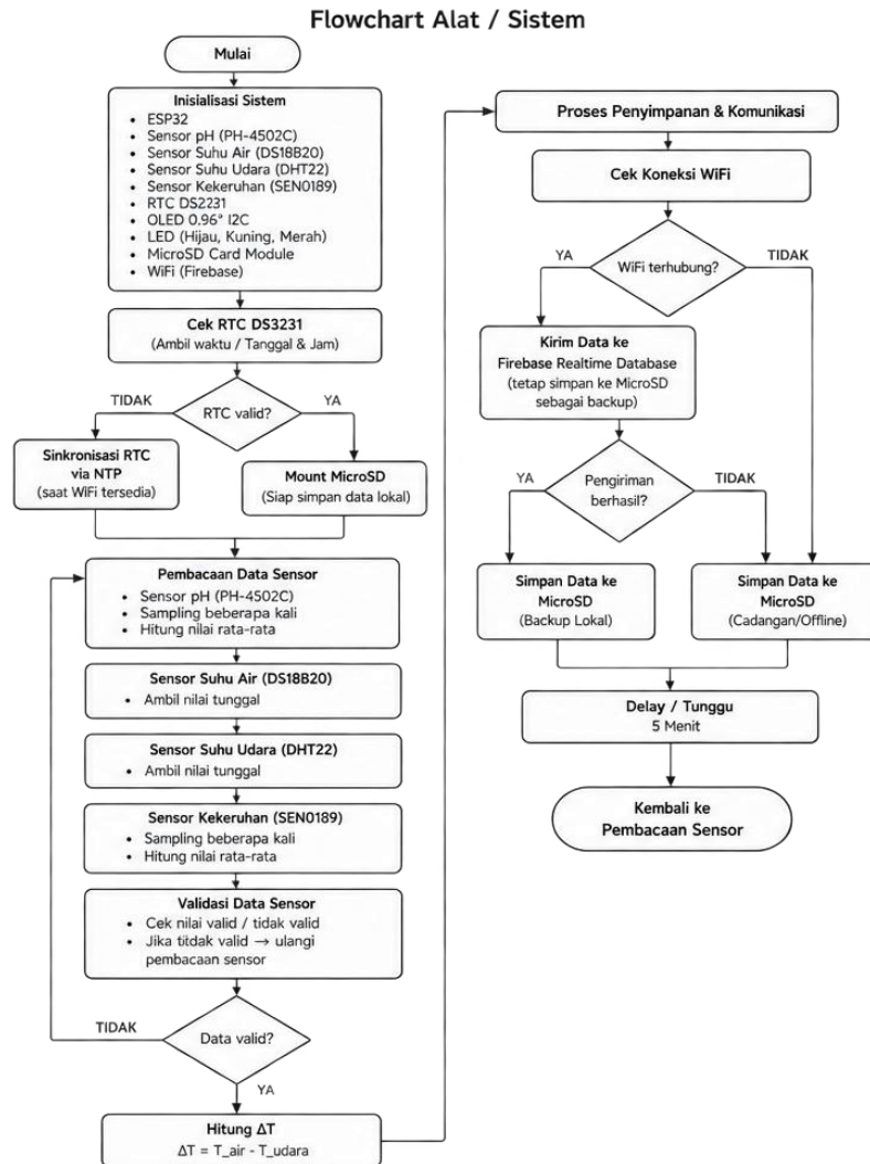
Gambar 3. 3 Flowchart Sistem
