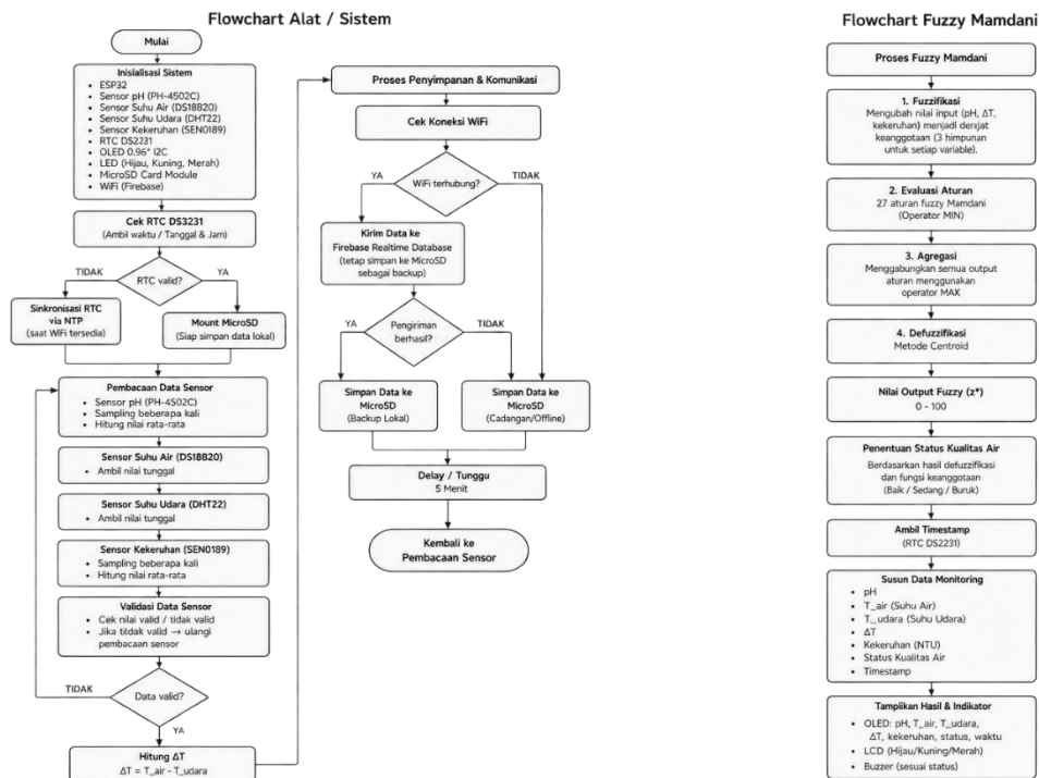
Gambar 3. 3 Flowchart Sistem
