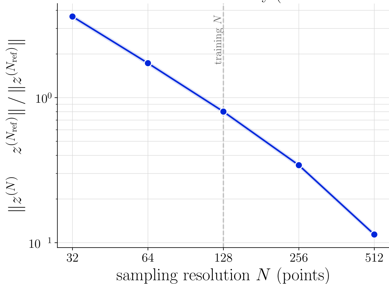
Encoder discretization-consistency (reference N=1024 )
