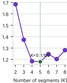
Davies-Bouldin (lower is better)
