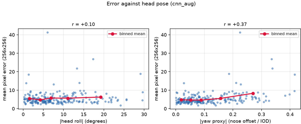
Figure 11: Error against head pose: roll is flat, yaw is not.
