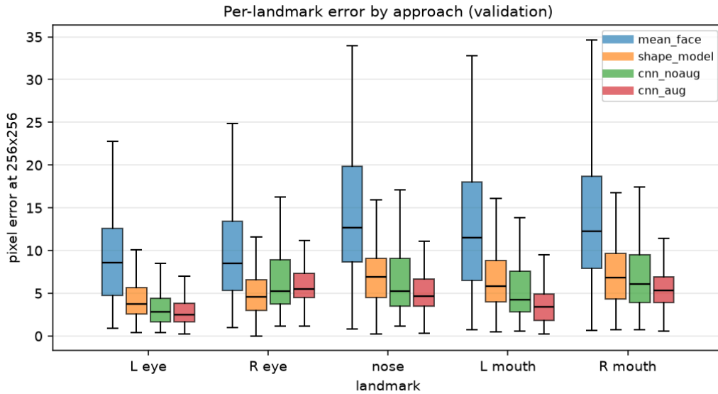
Figure 8: Per-landmark error.
