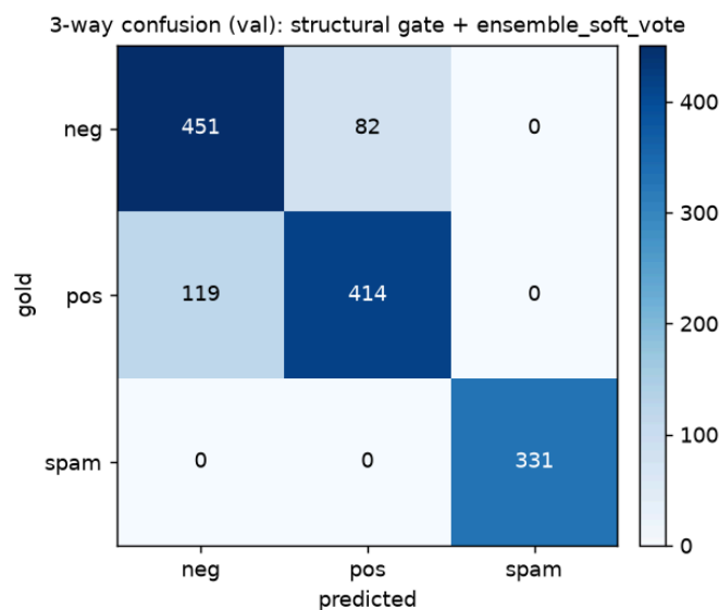
Figure 3: Three-way validation confusion matrix, deployed system.
