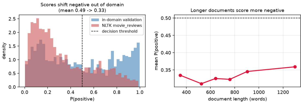
Figure 4: Scores shift negative out of domain (left) and fall with document length (right), explaining the asymmetric recall in Figure 5.
