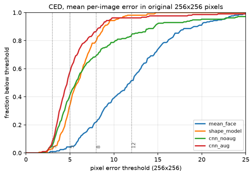
Figure 7: CED in original-resolution pixels, graded thresholds marked. The crossing curves are the fat tail made visible.
