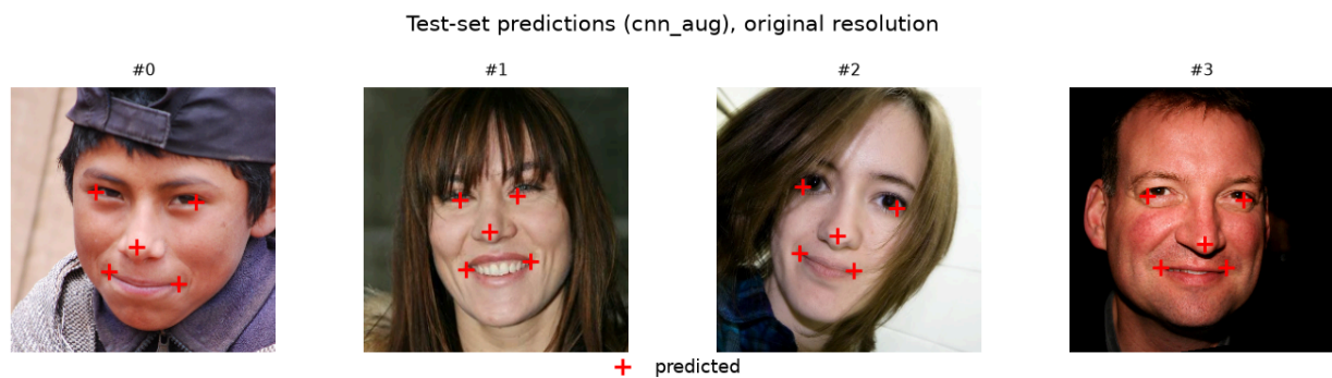
Figure 13: First four test images with predicted landmarks at original resolution.
