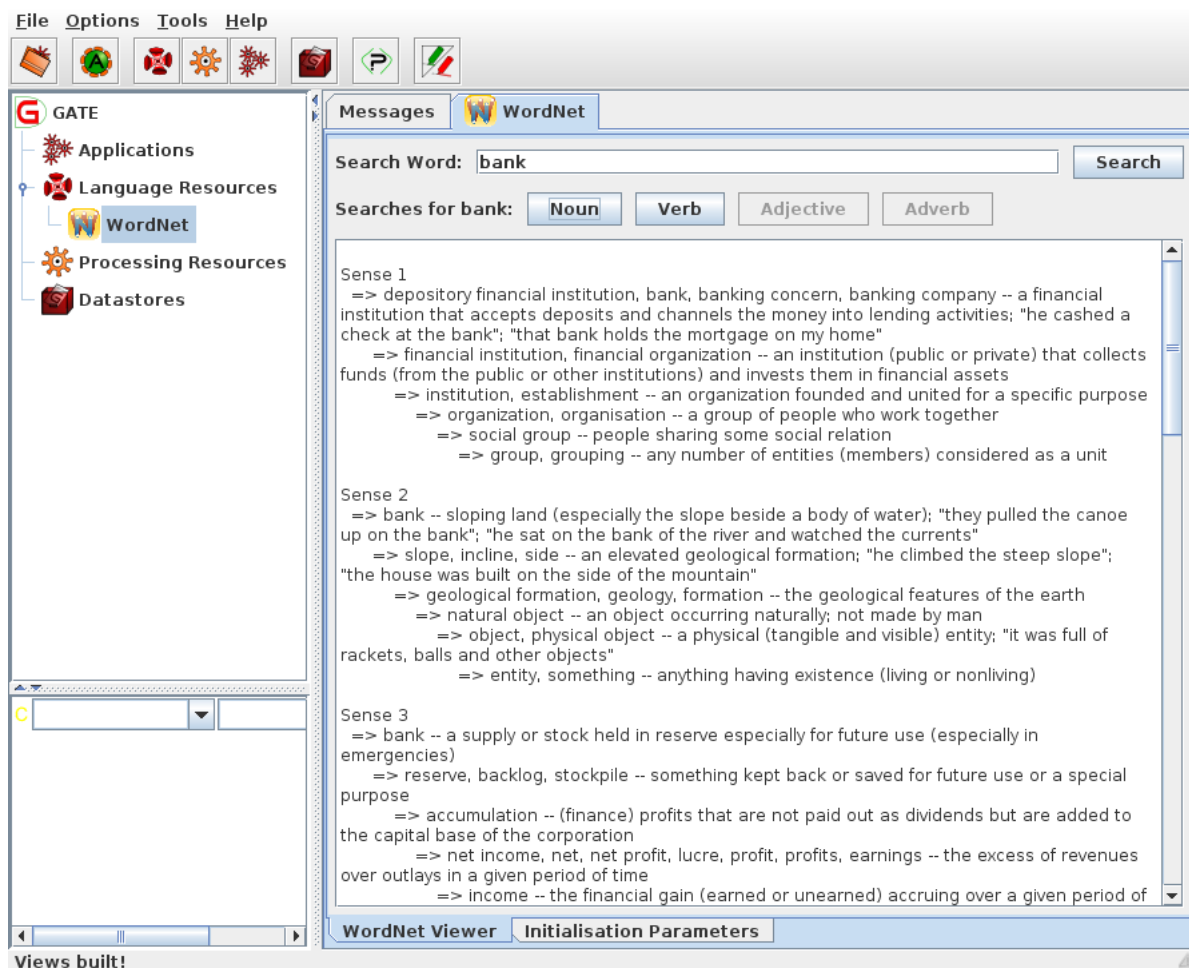
Figure 21.7: WordNet in GATE
