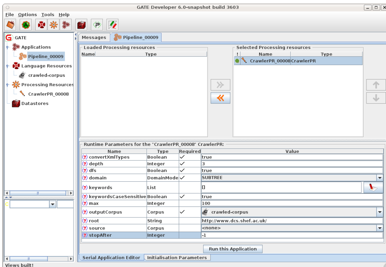
Figure 21.5: Crawler parameters
