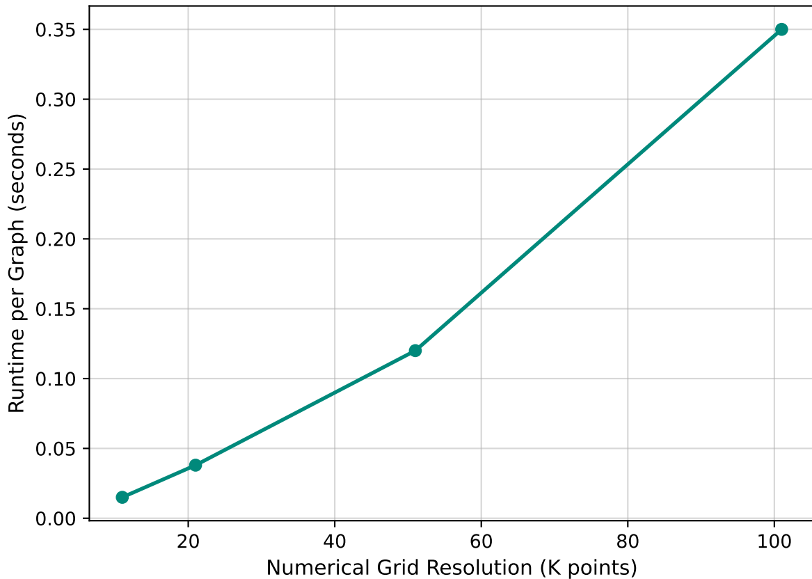
Figure 13: Grid Resolution vs. Inference Runtime
