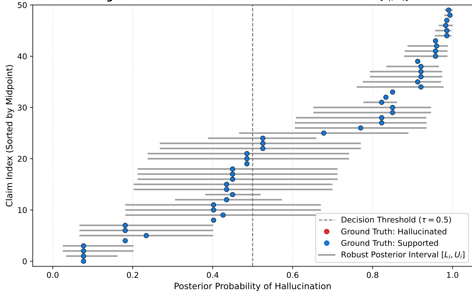
Figure 2: Standard BP vs. Robust Posterior Intervals [L_i, U_i]
