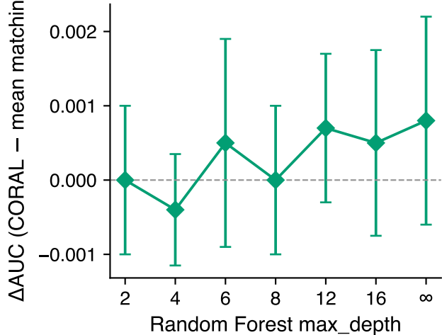
(b) Covariance-alignment gain vs depth
