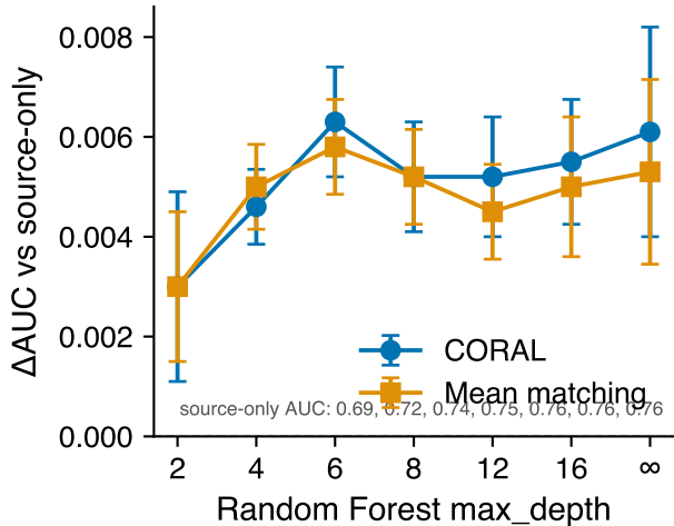
(a) DA benefit vs tree depth
