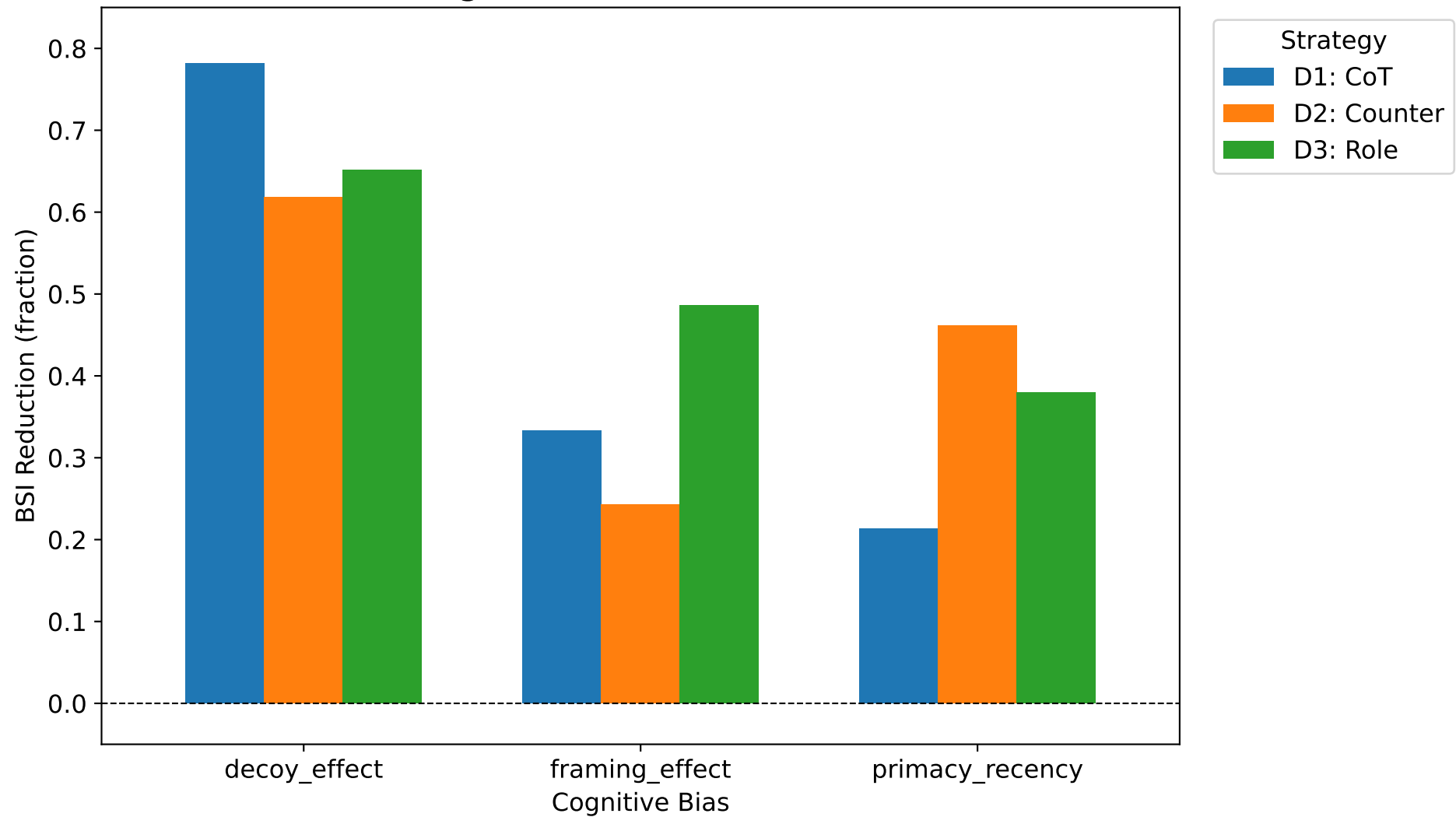
Debiasing Effectiveness — llama-3.1-8b
