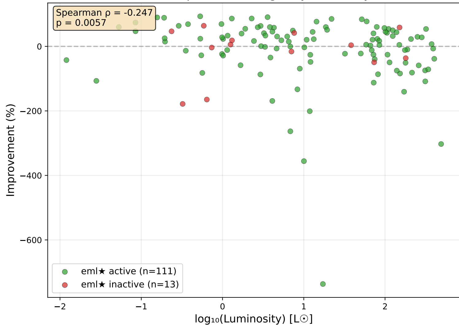
eml★ improvement vs galaxy luminosity
