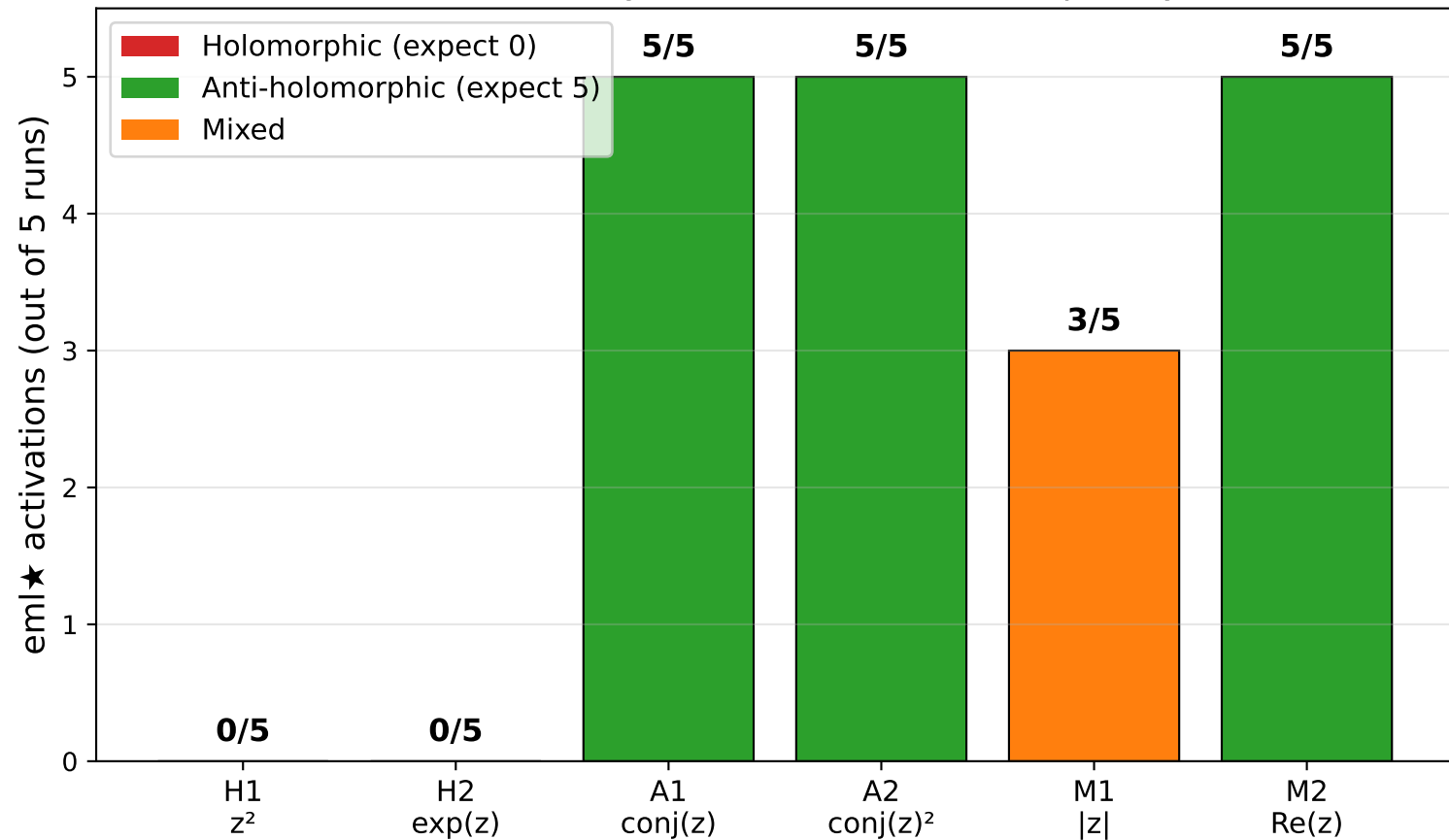
Characterization battery: eml★ as non-holomorphicity detector
