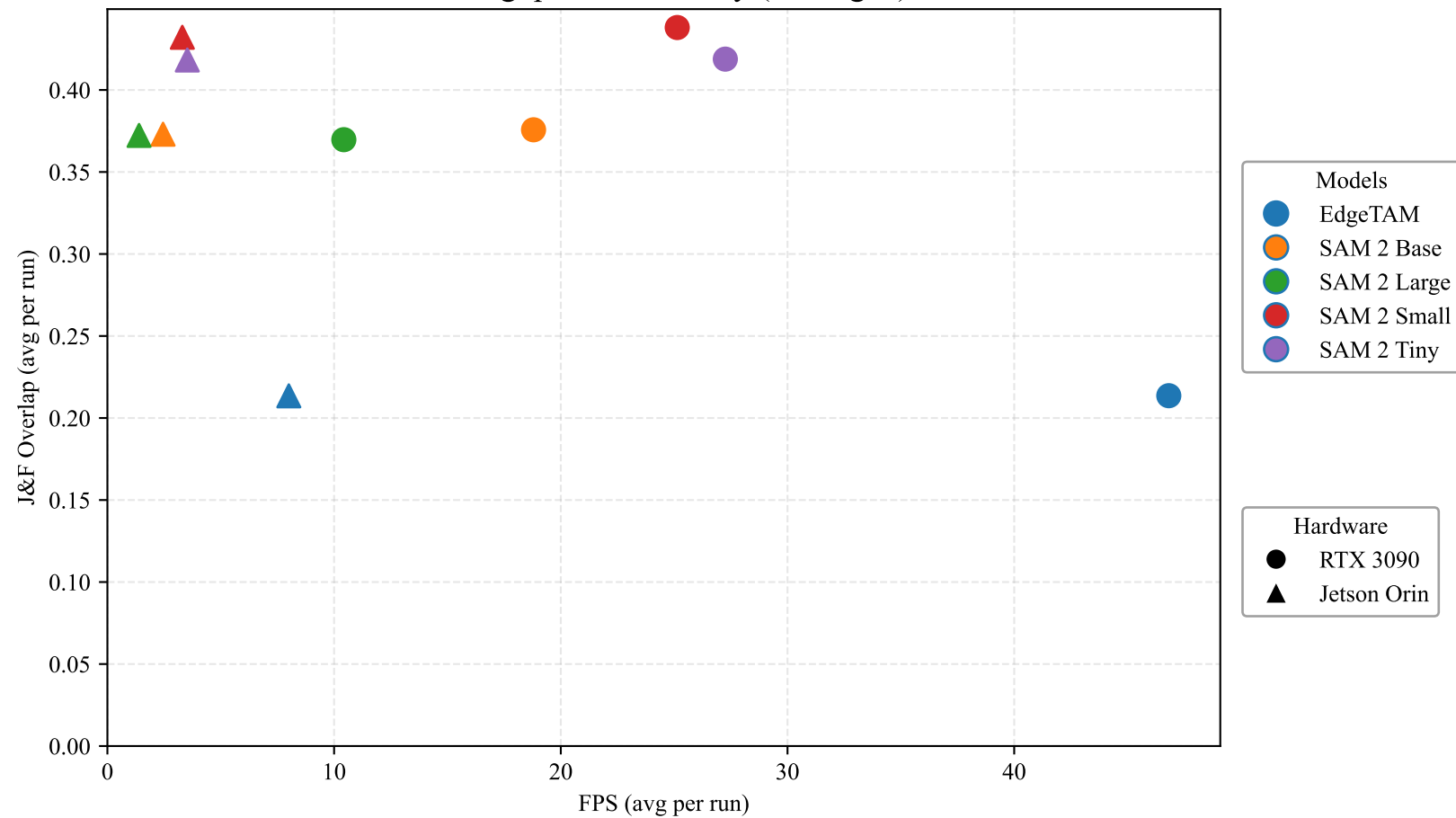
Throughput vs Accuracy (Averaged)
