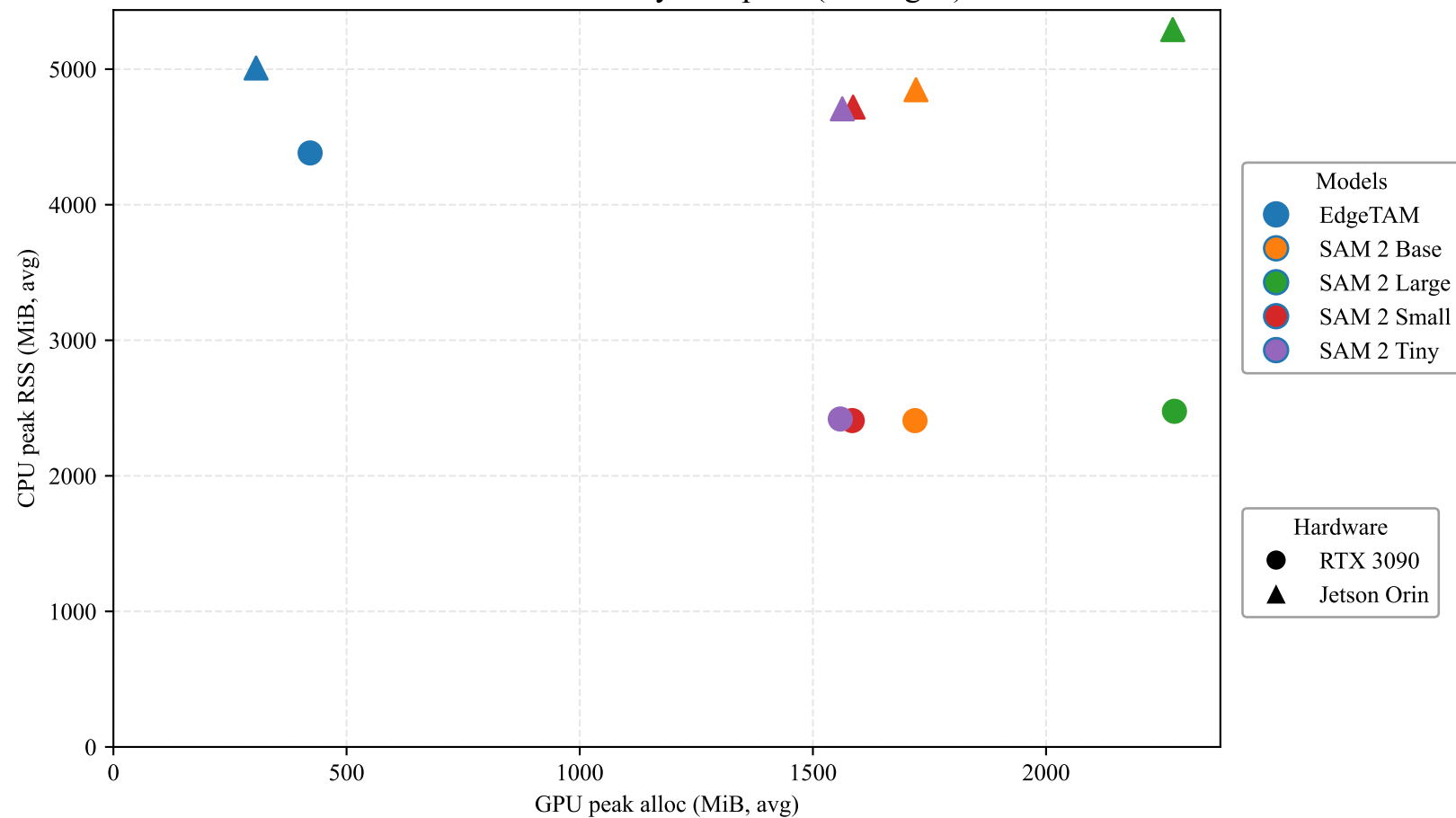
GPU vs CPU Memory Footprint (Averaged)
