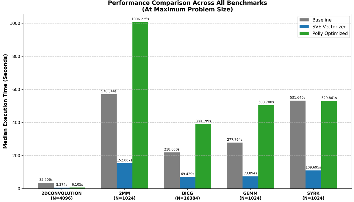
Figure 1: Performance metrics of the evaluated kernels.
