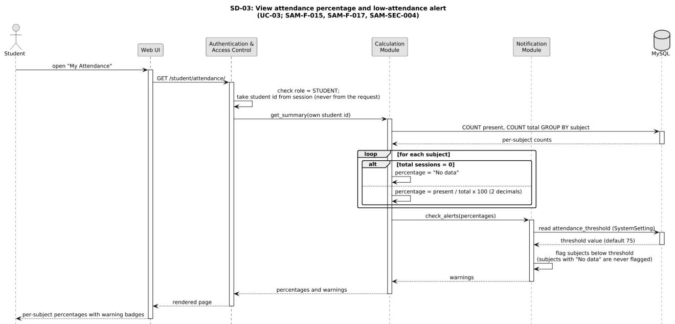
Figure 4.4 — SD-03: View attendance percentage and low-attendance alert
