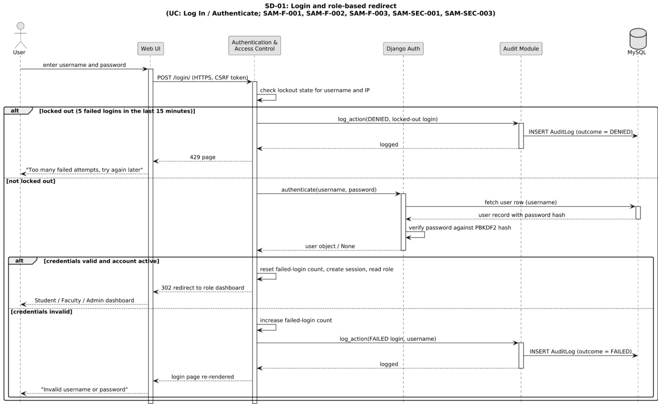
Figure 4.2 — SD-01: Login and role-based redirect
