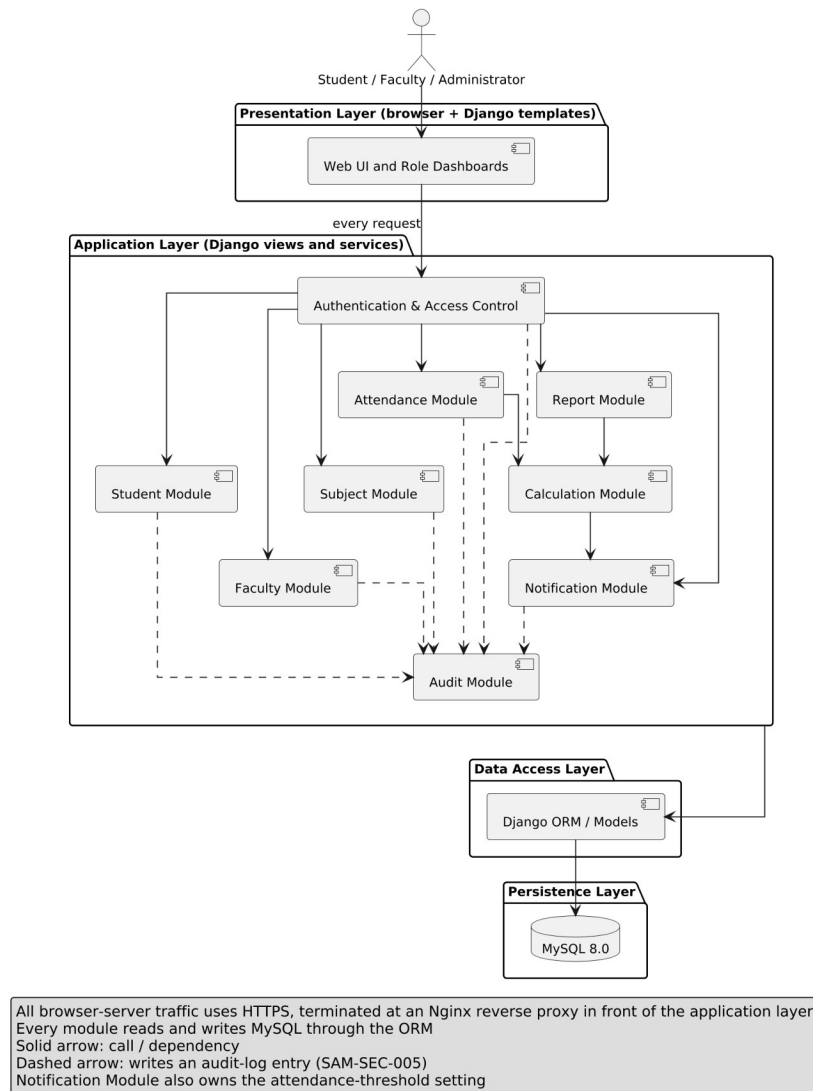
Figure 3.1 — SAMS UML component diagram (layered architecture)
