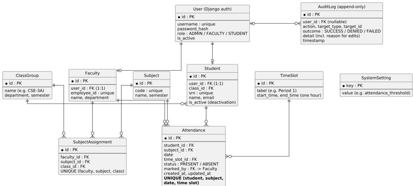
Figure 4.1 — SAMS entity-relationship diagram
