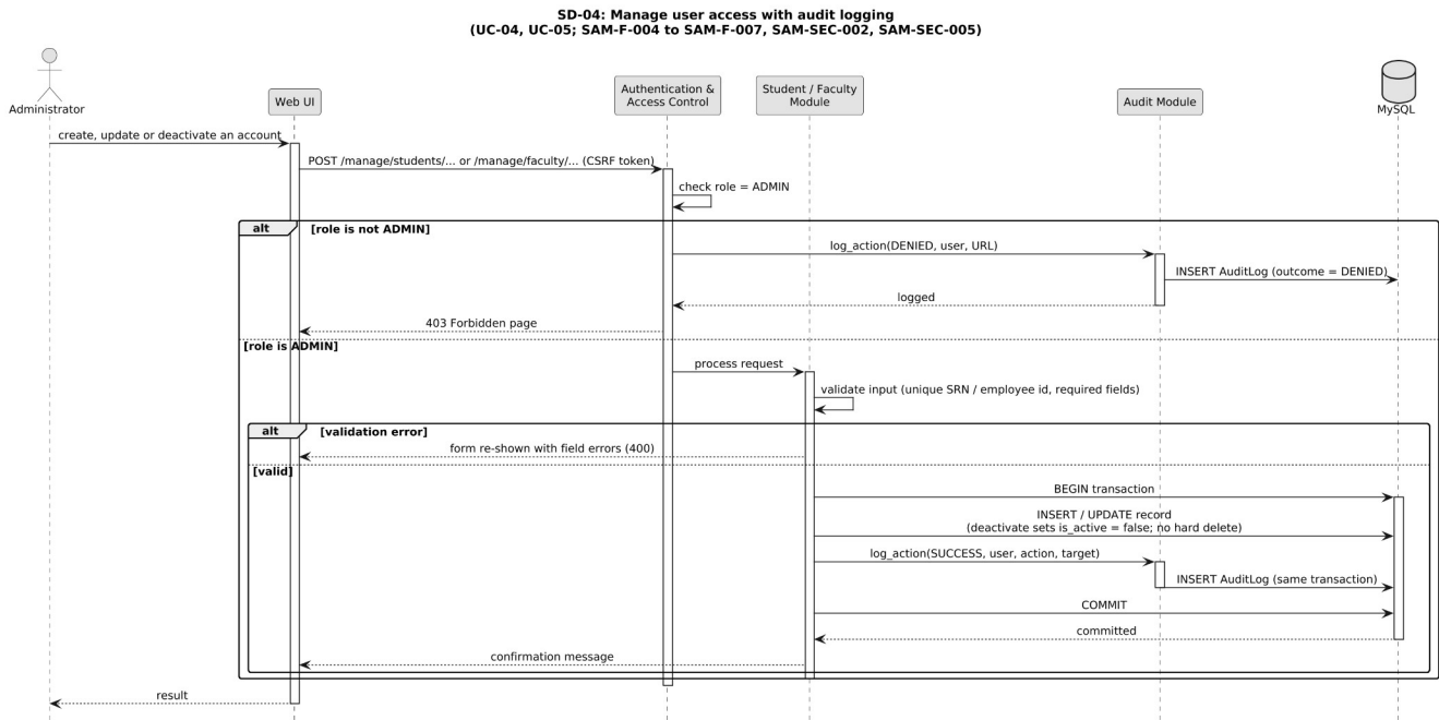
Figure 4.5 — SD-04: Manage user access with audit logging
