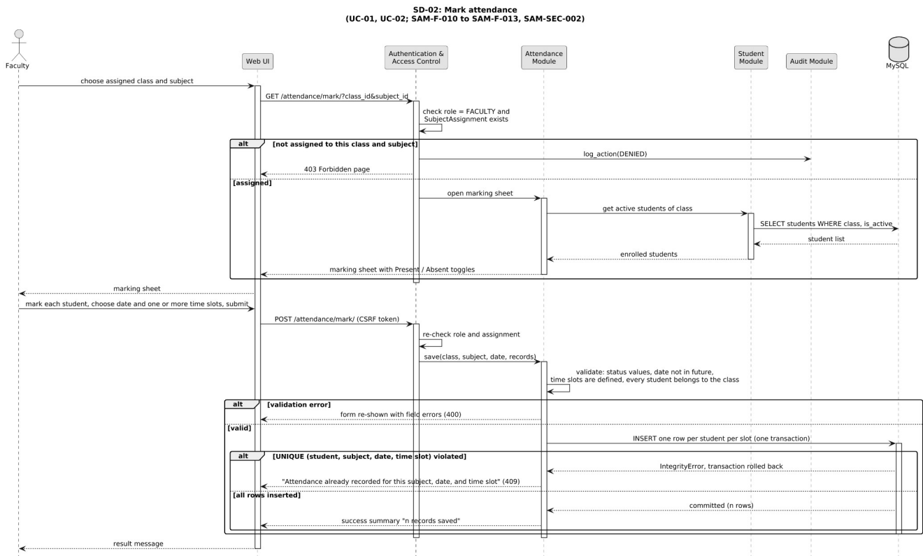
Figure 4.3 — SD-02: Mark attendance
