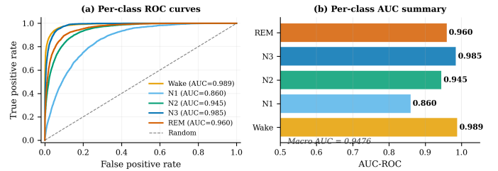
Fig. 4. Receiver operating characteristic (ROC) curves and AUC per sleep stage. One-vs-rest classification.
