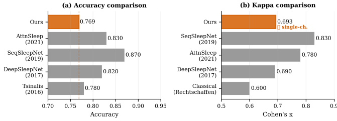
Fig. 5. Comparison with published methods on Sleep-EDF dataset. Orange = this study (single-channel EEG Fpz-Cz).
