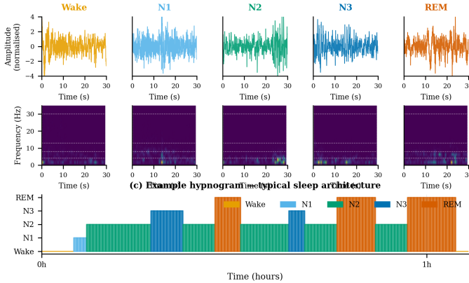
Fig. 6. EEG characteristics per sleep stage. Row 1: raw signal. Row 2: time-frequency spectrogram. Row 3: example hypnogram showing typical sleep cycle architecture.
