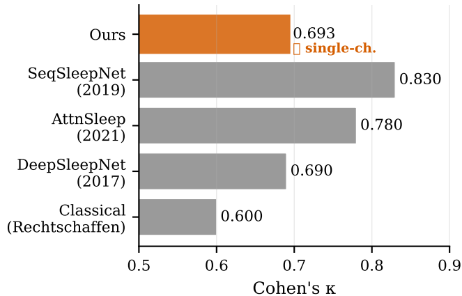
Fig. 5. Comparison with published methods on Sleep-EDF dataset. Orange = this study (single-channel EEG Fpz-Cz).
