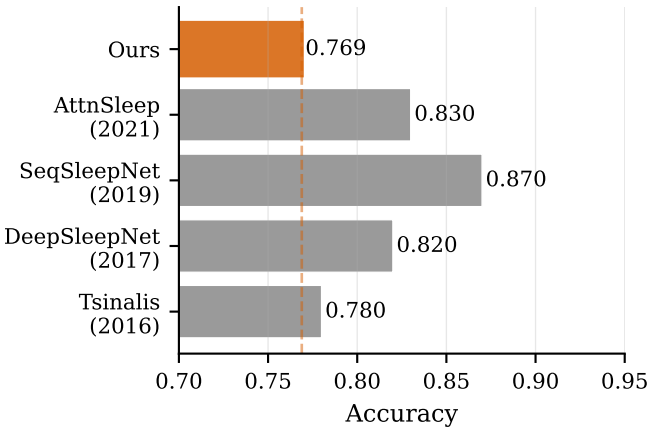
Fig. 5. Comparison with published methods on Sleep-EDF dataset. Orange = this study (single-channel EEG Fpz-Cz).
