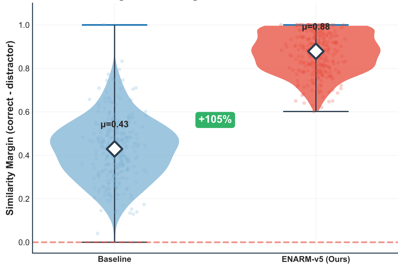
Figure 6: Ranking Confidence Distribution
