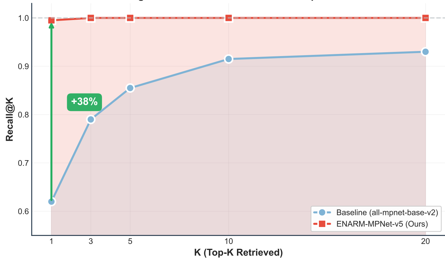
Figure 4: Retrieval Performance Comparison
