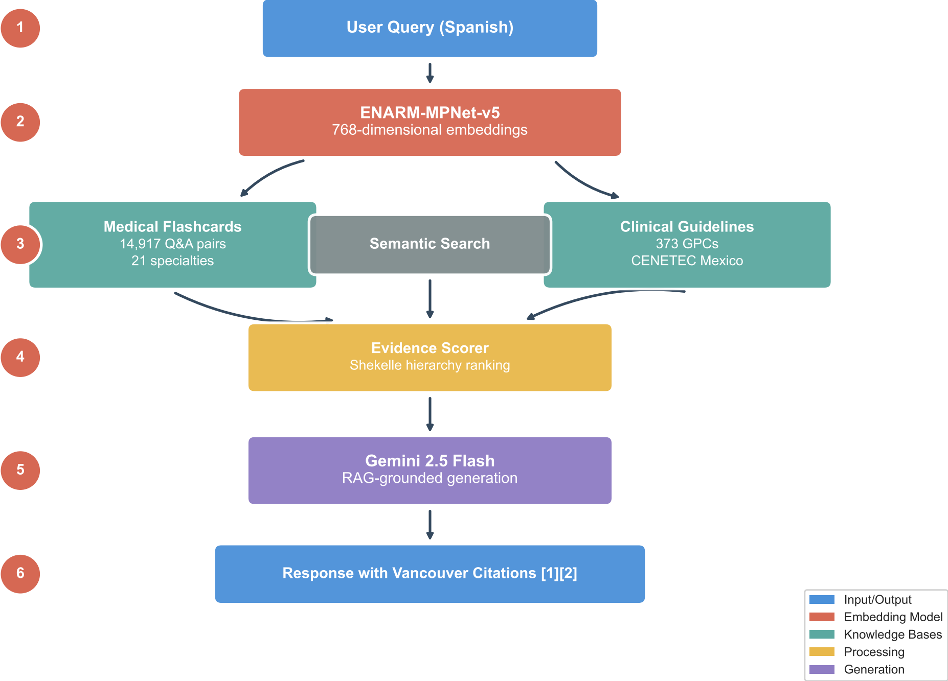
Figure 1: ENARM-MPNet RAG System Architecture
