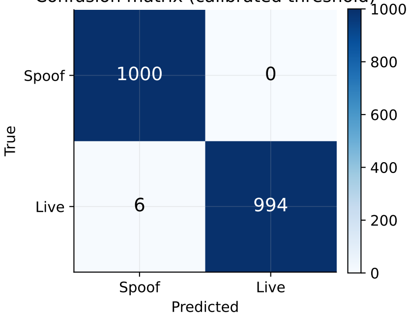
Confusion matrix (calibrated threshold)
