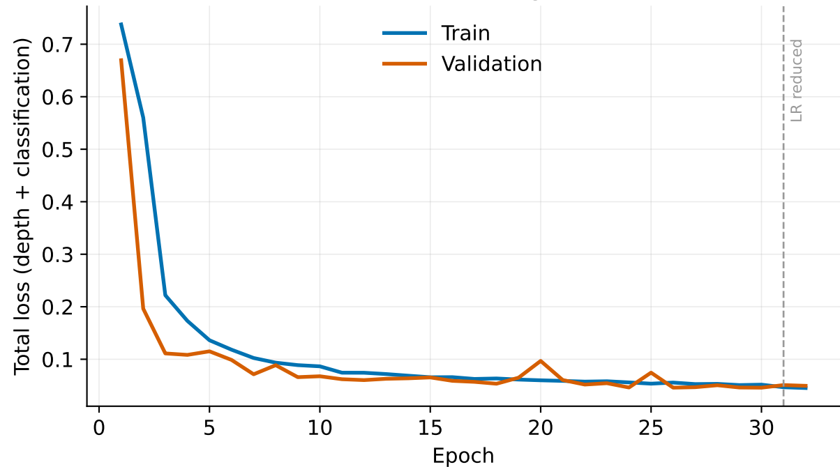
CDCN++ training loss
