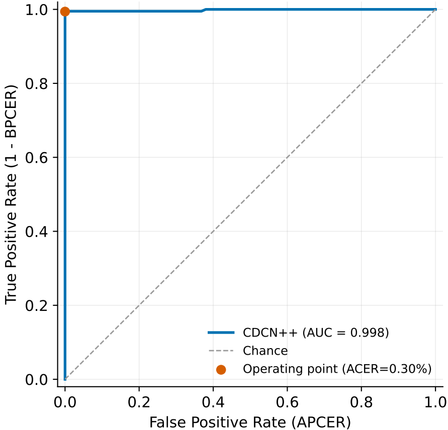
ROC curve on held-out CelebA-Spoof validation set
