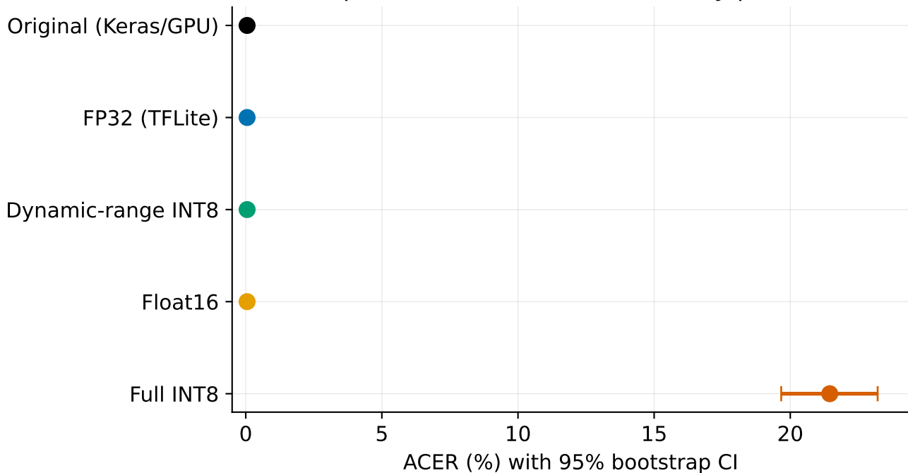
ACER point estimate and uncertainty per variant
