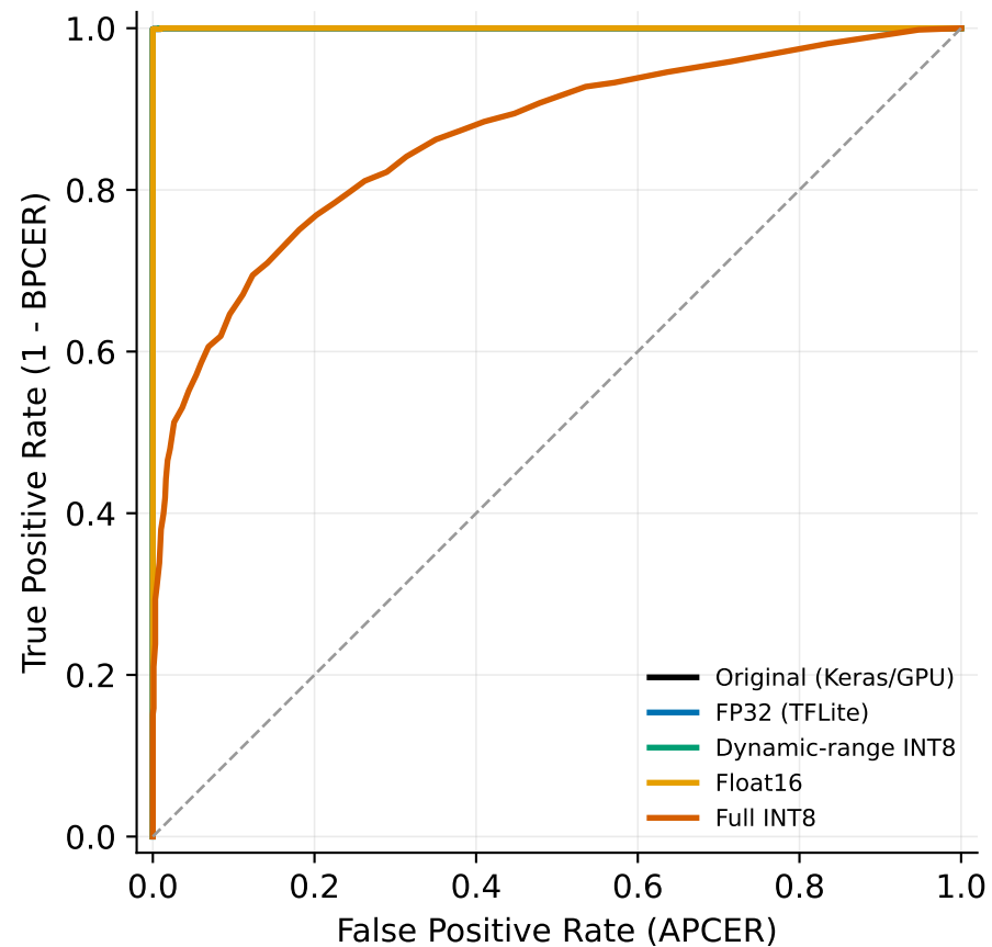
ROC curves
