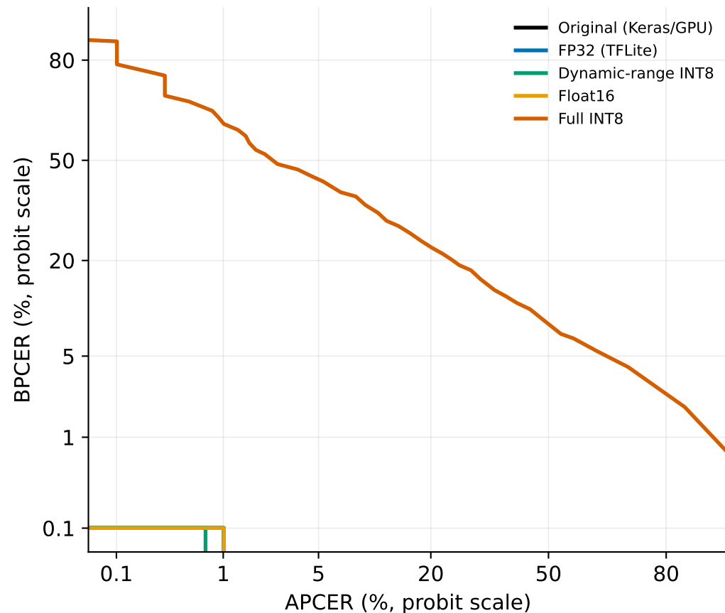
DET curves
