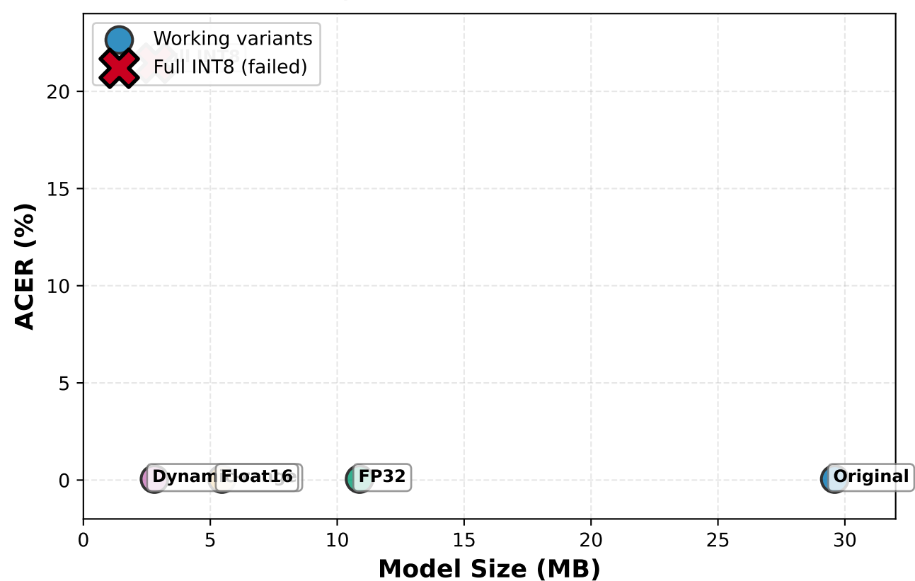
(b) Size-Accuracy Trade-off: INT8 Quantization Failure
