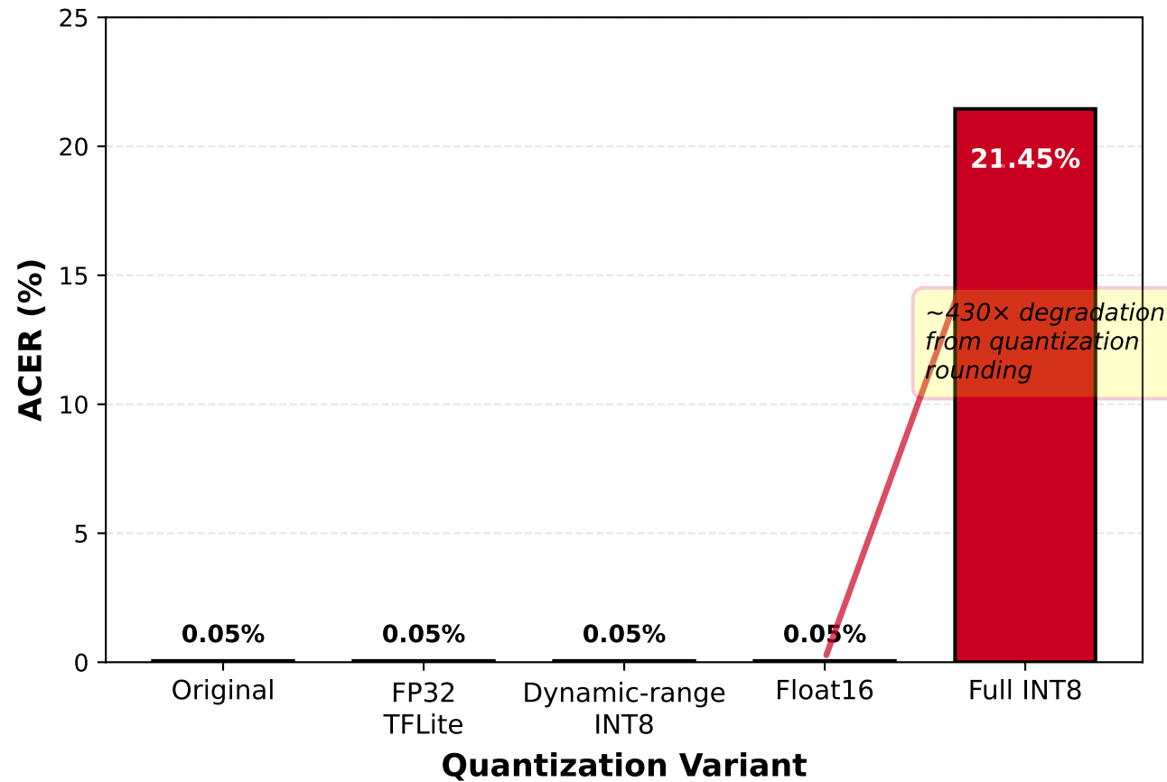
(a) Quantization Collapse: ACER Performance
