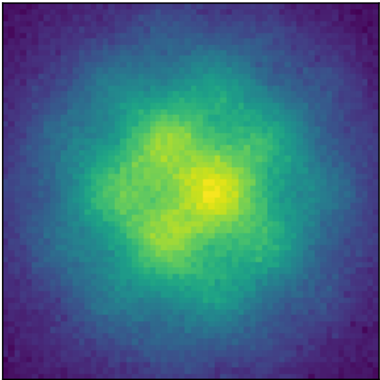
Predicted Depth
