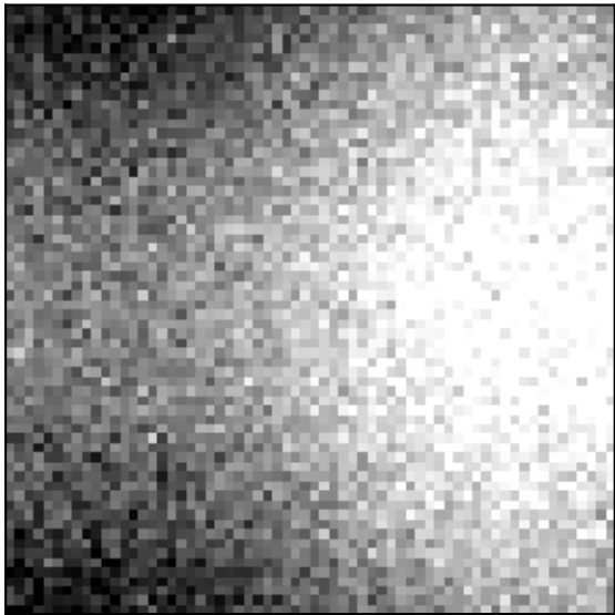
Input Image
