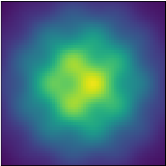
Ground-truth Depth
