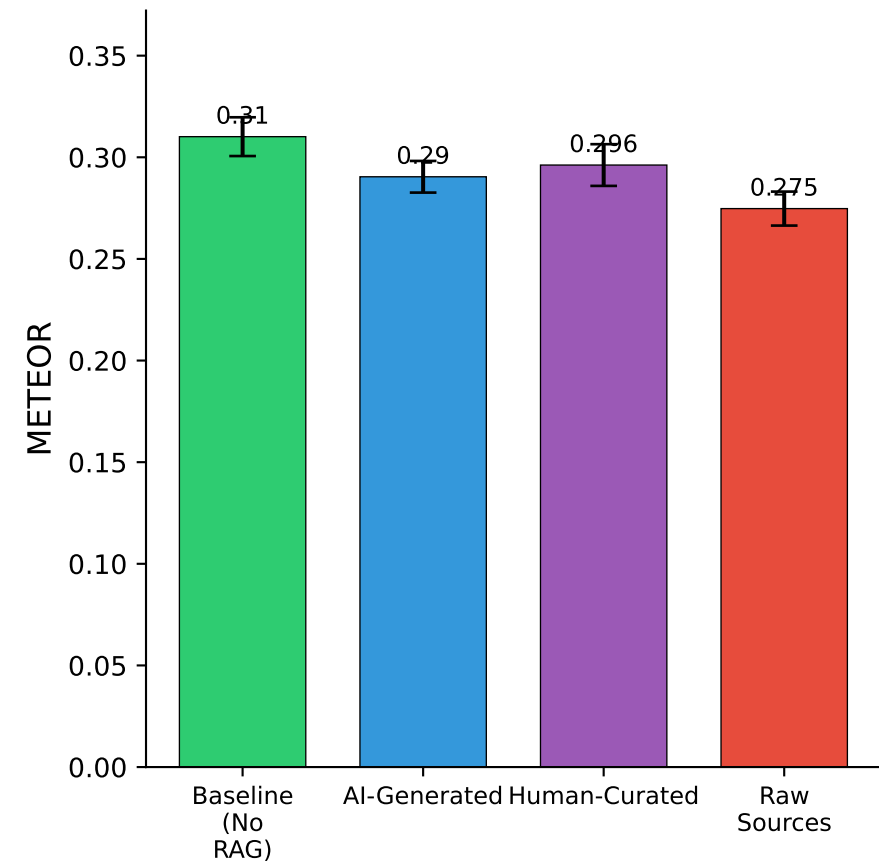
METEOR
