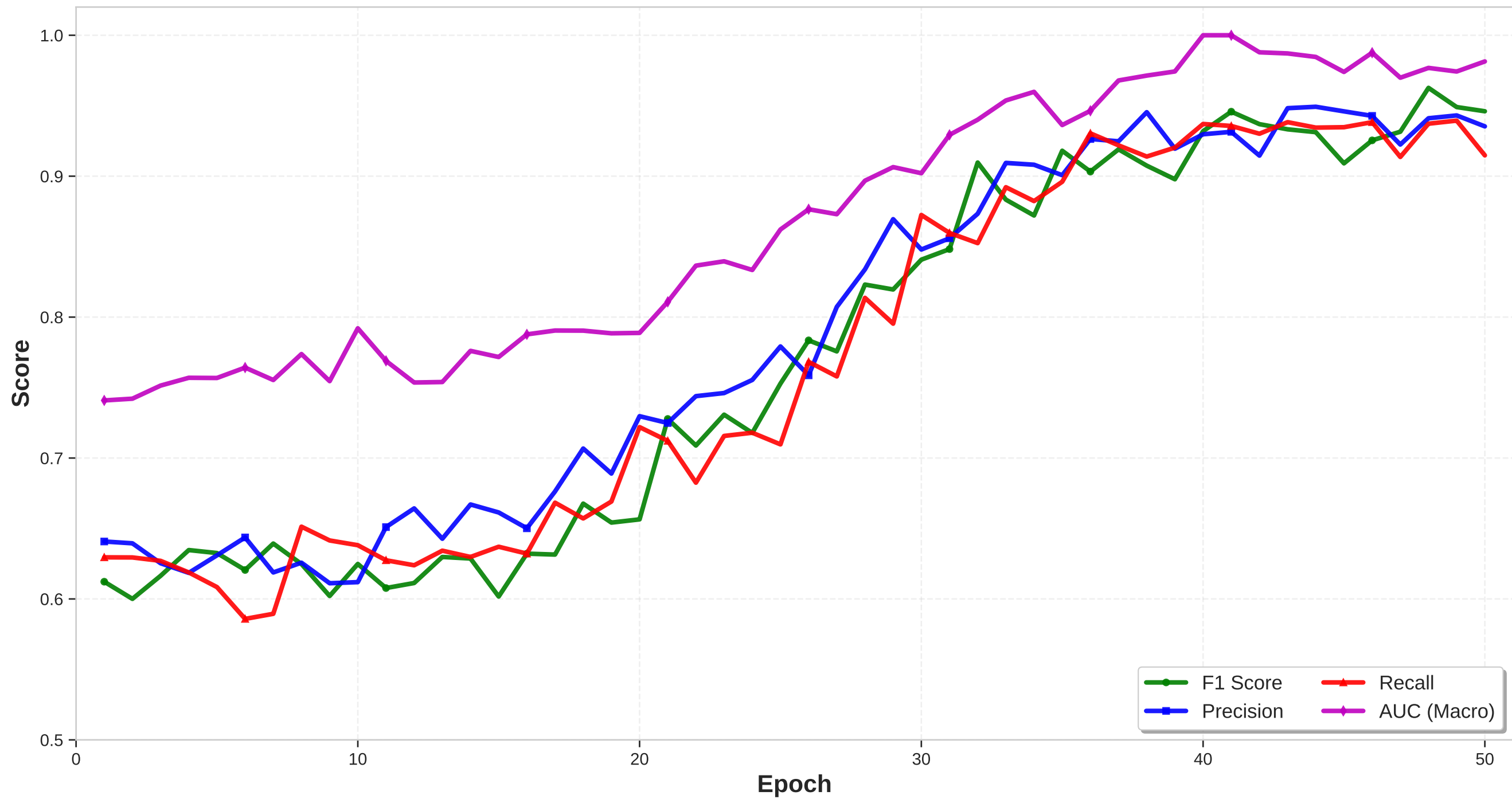
Performance Metrics Over Training
