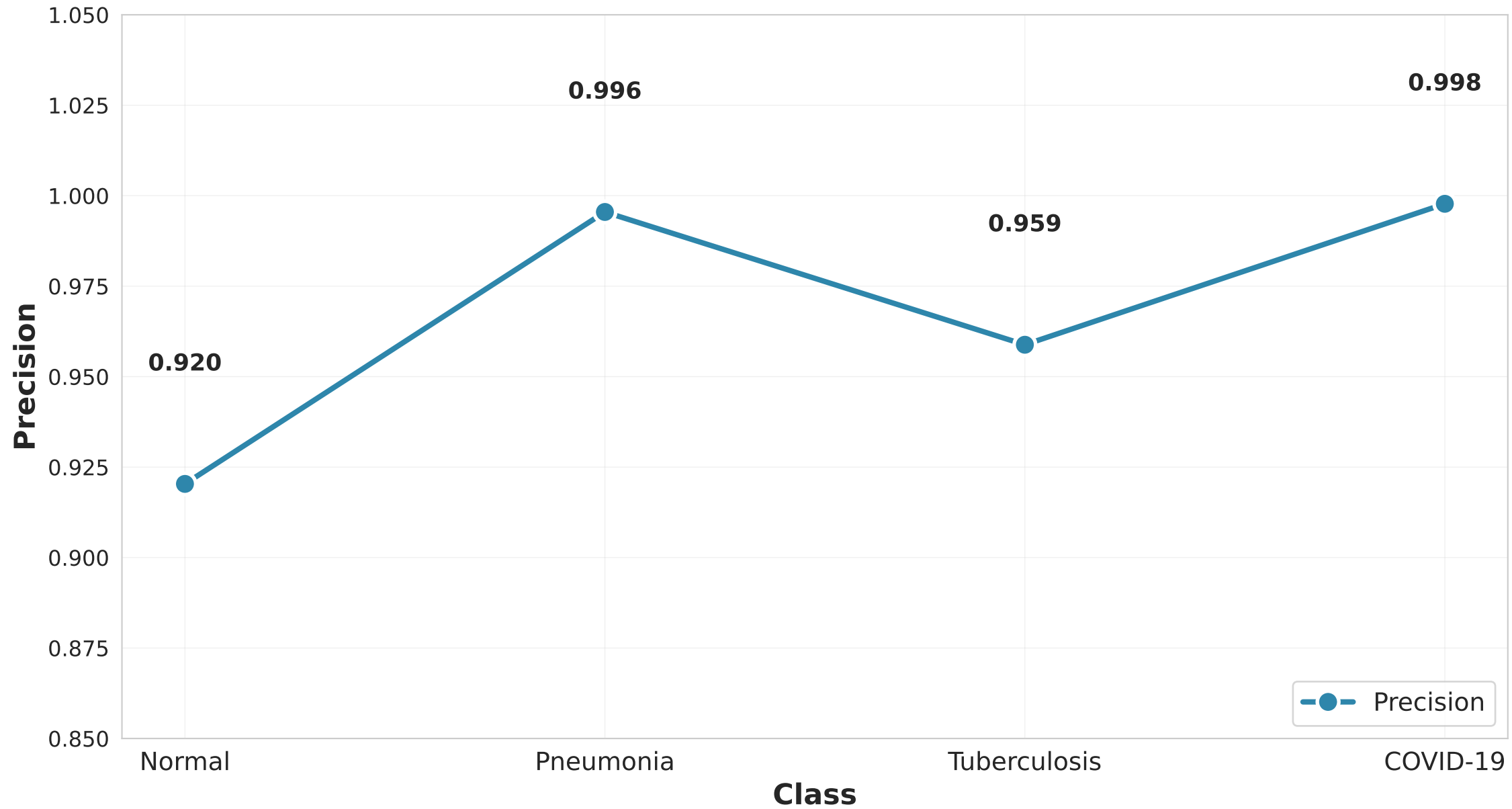
Precision by Class
