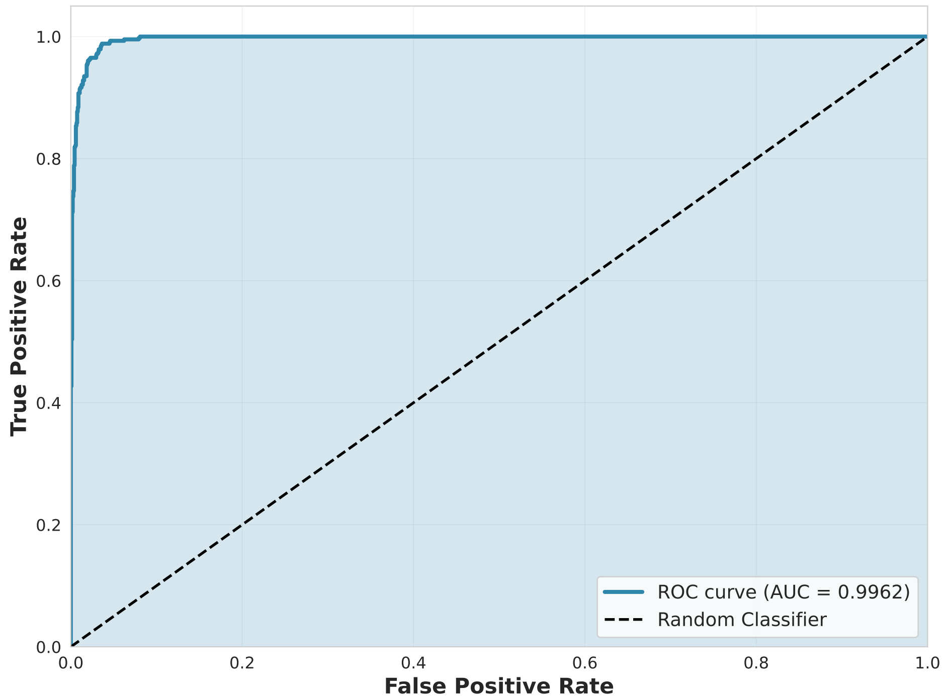
ROC Curve - Normal
