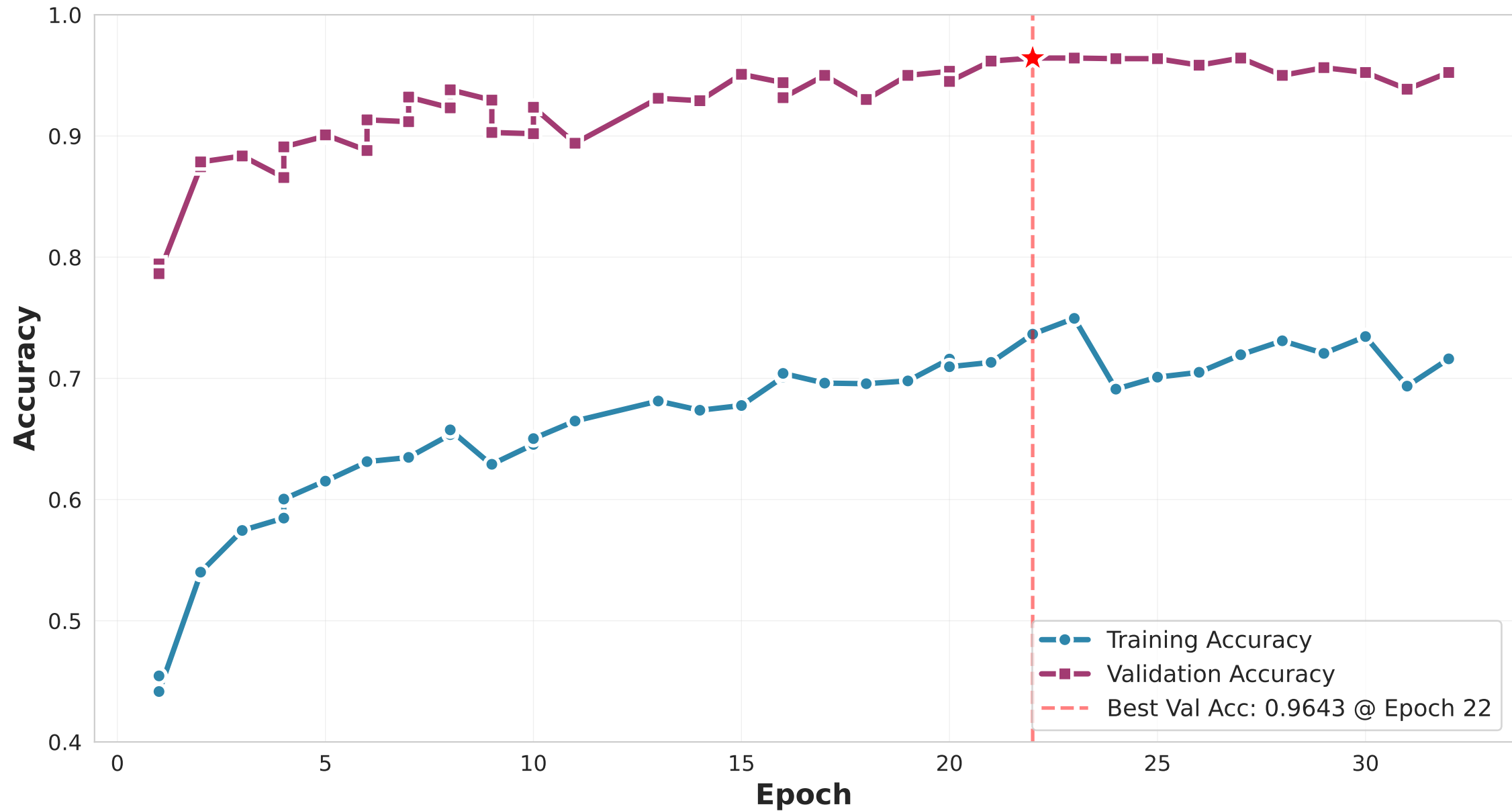
Training & Validation Accuracy Over Epochs
