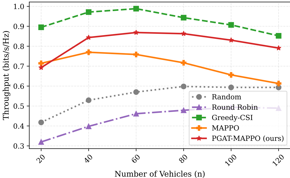
Throughput vs. Number of Vehicles
