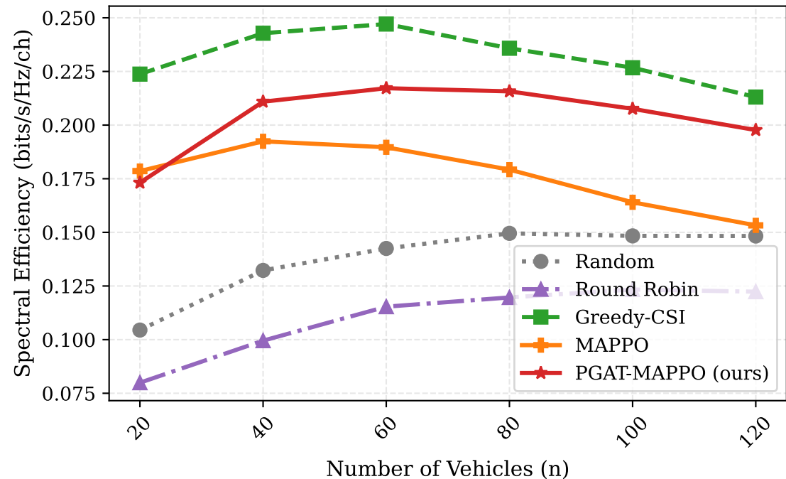
Spectral Efficiency vs. Number of Vehicles
