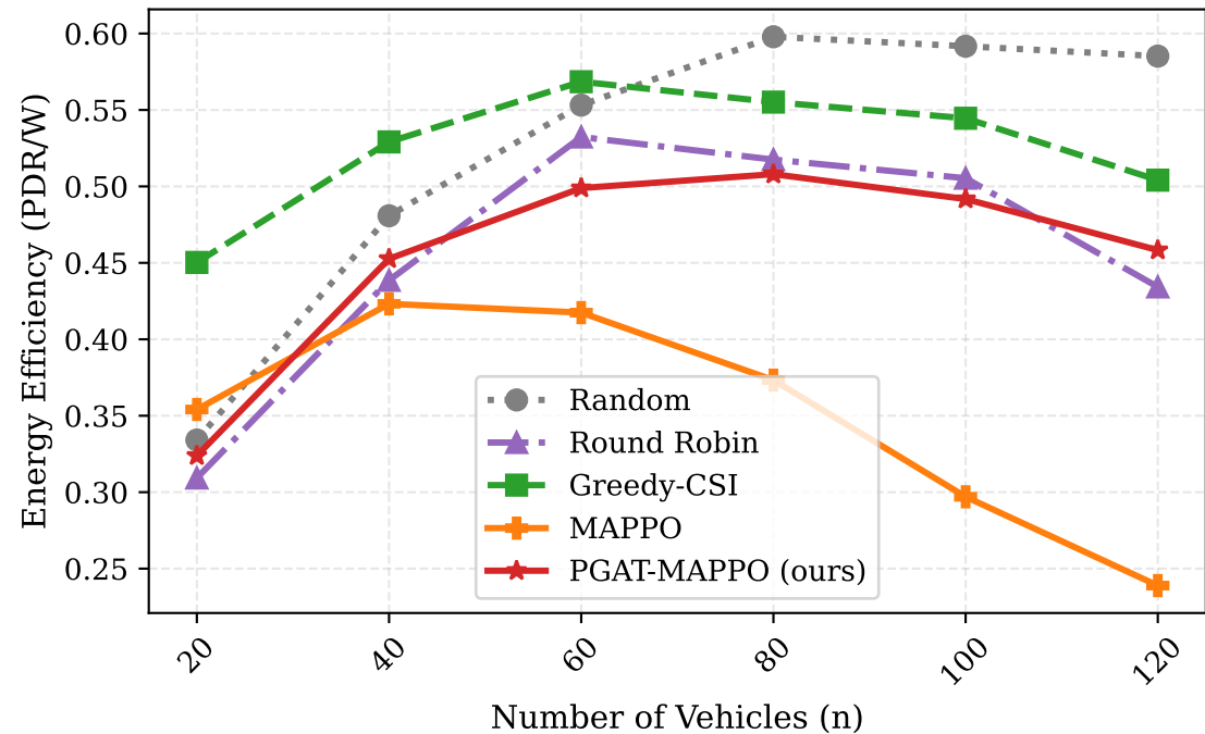
Energy Efficiency vs. Number of Vehicles
